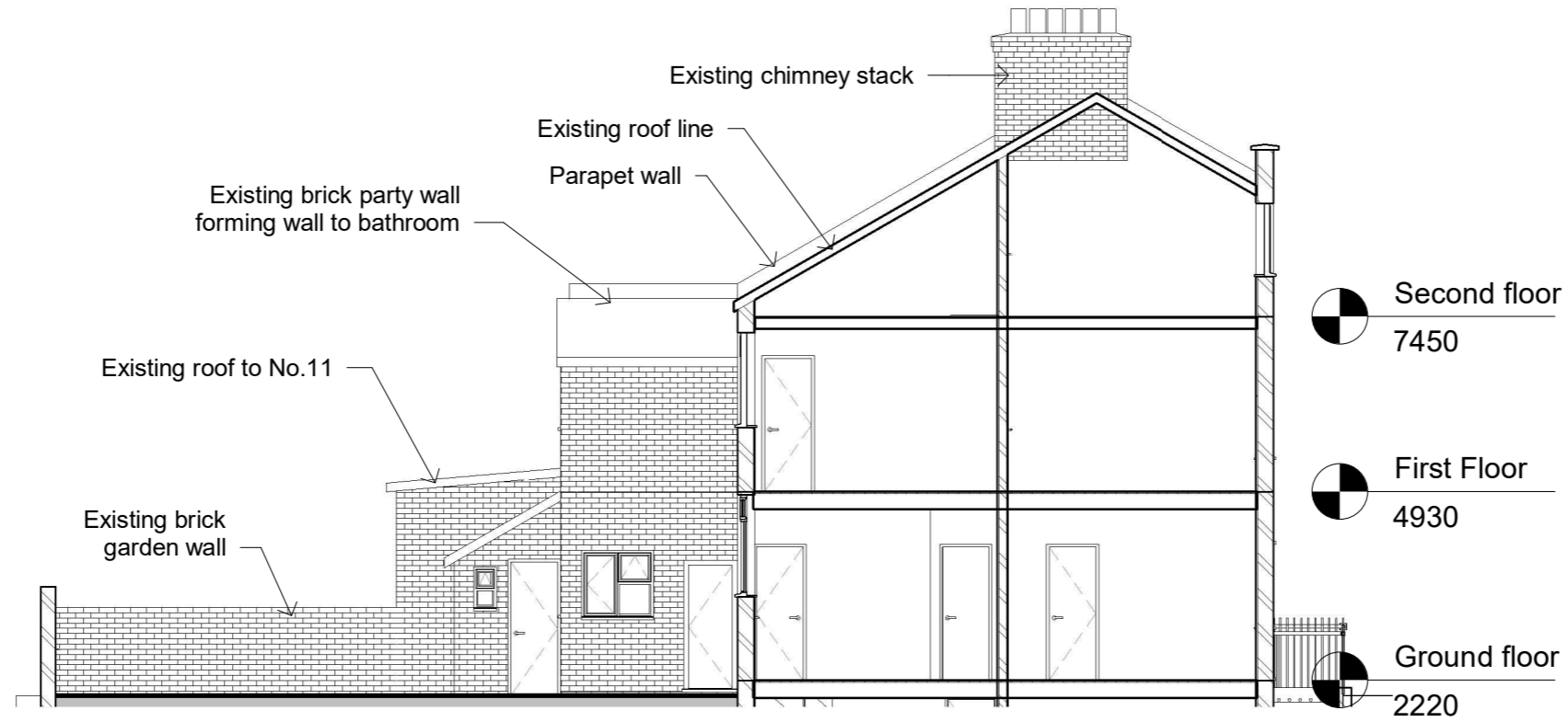
Section from No.11 Oxford Street
