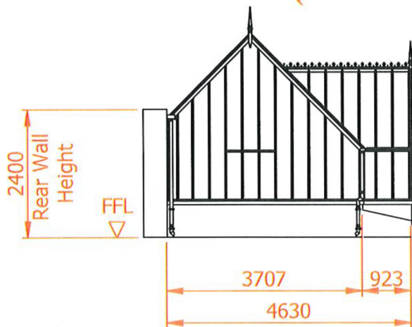
East Elevation
