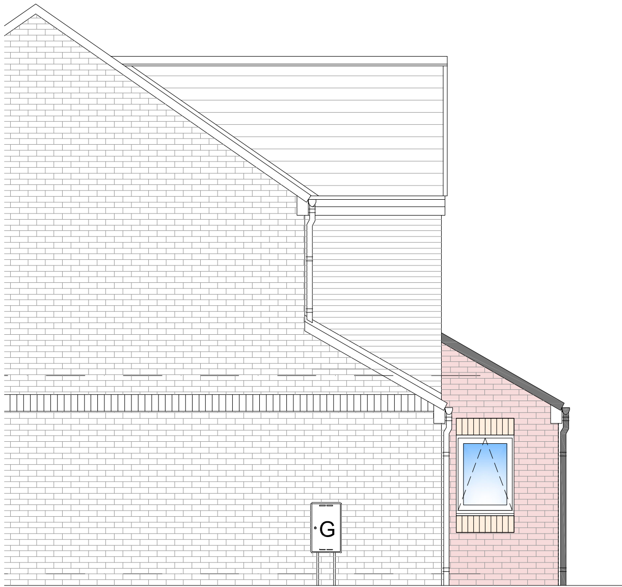
NORTH SIDE ELEVATION (as Proposed) 1:50 @ A3
