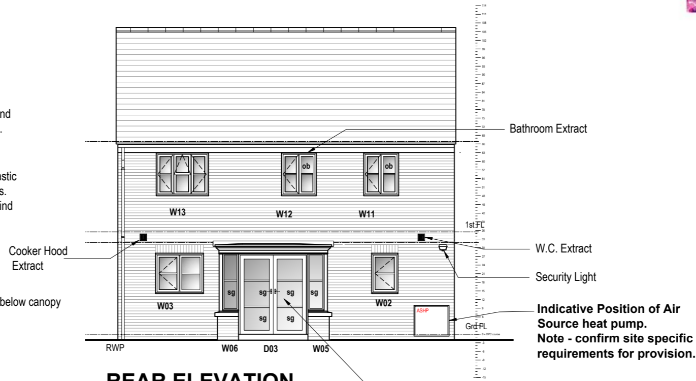
REAR ELEVATION
