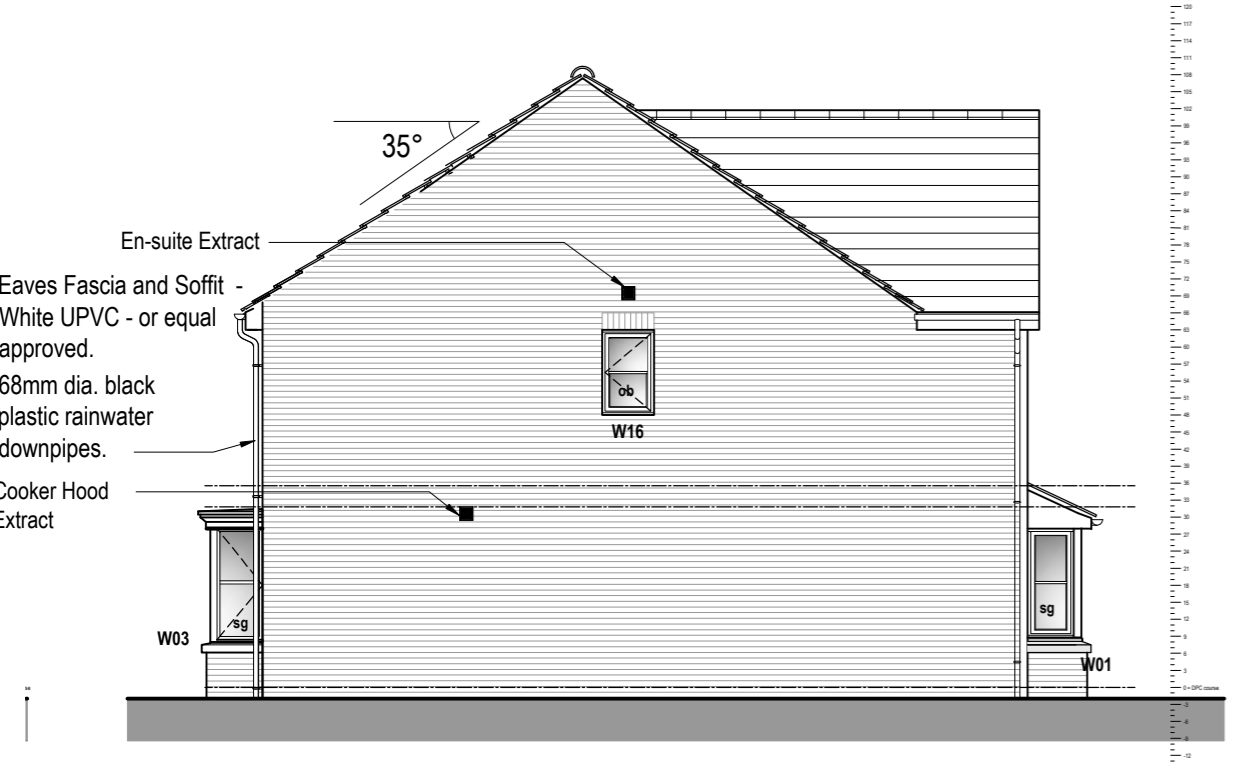
LEFT GABLE ELEVATION
