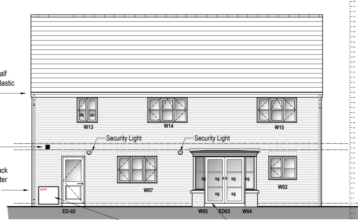
REAR ELEVATION
