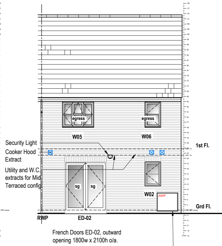
REAR ELEVATION
