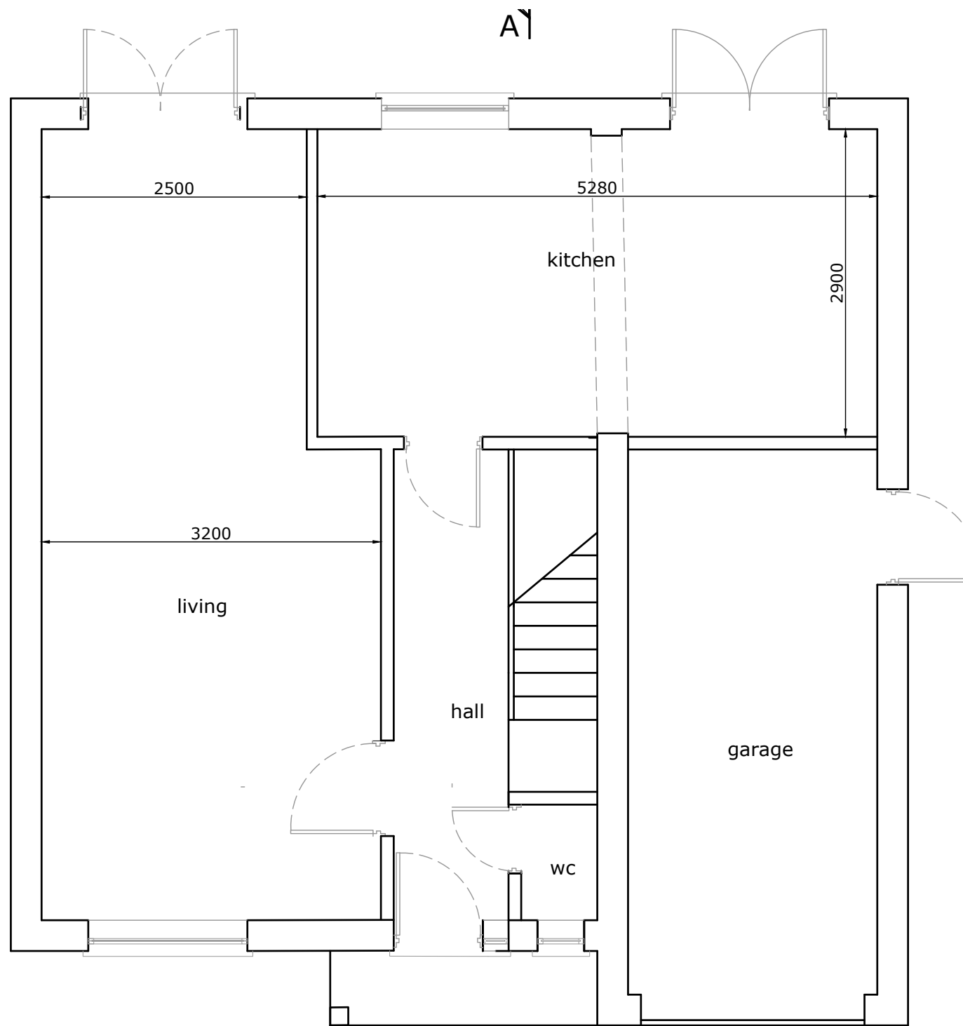
EXISTING GROUND FLOOR scale 1:50
