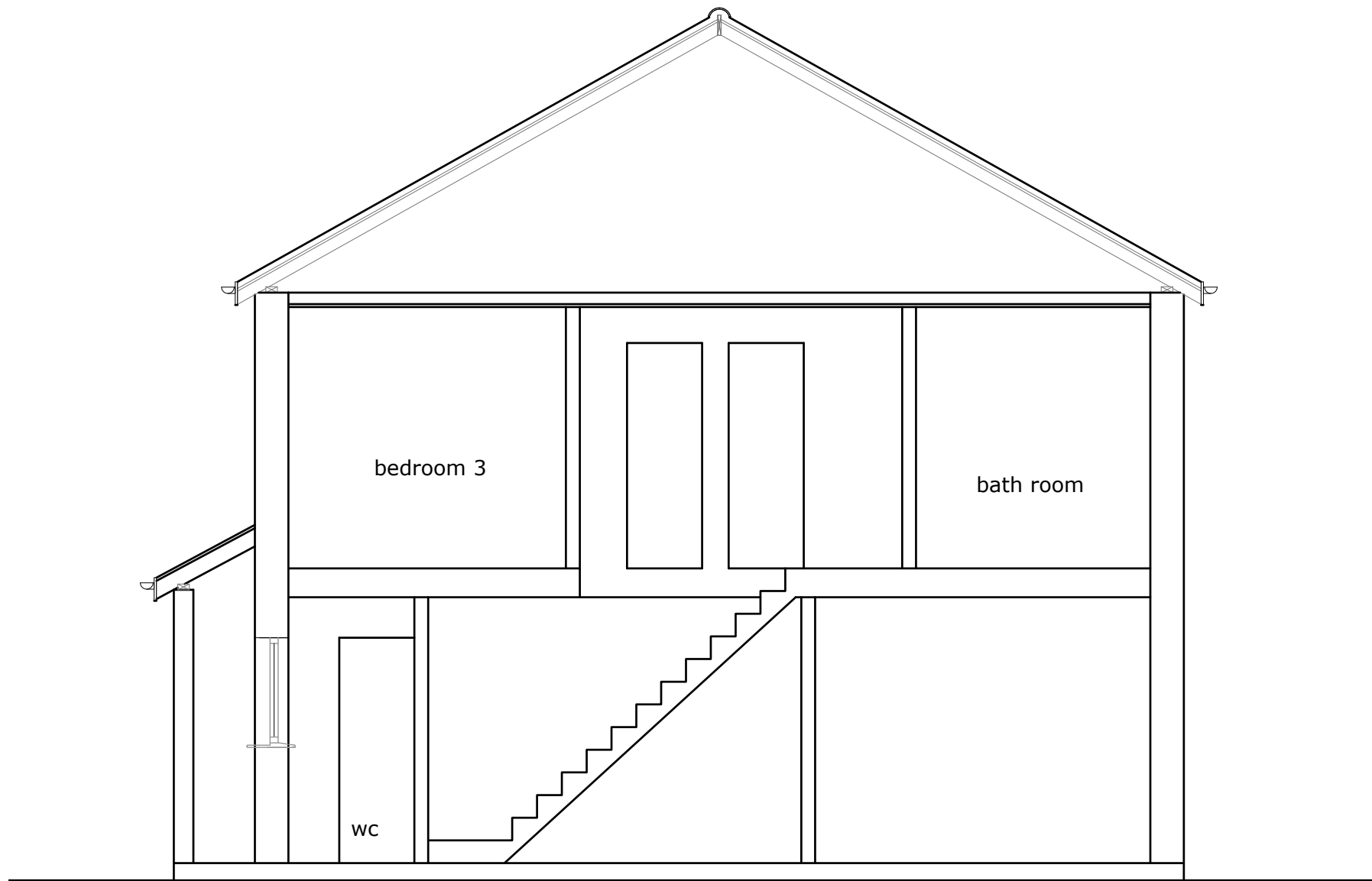
EXISTING SECTION A-A scale 1:50
