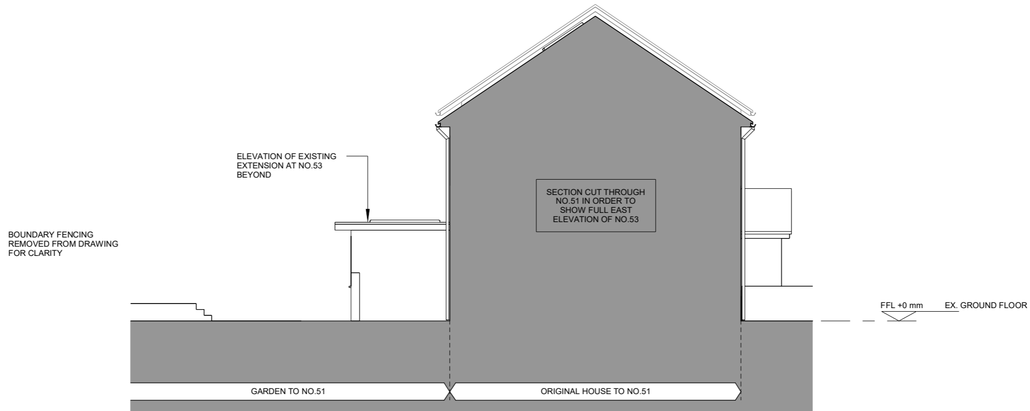
1 23095 - EXISTING EAST ELEVATION 1 : 100
