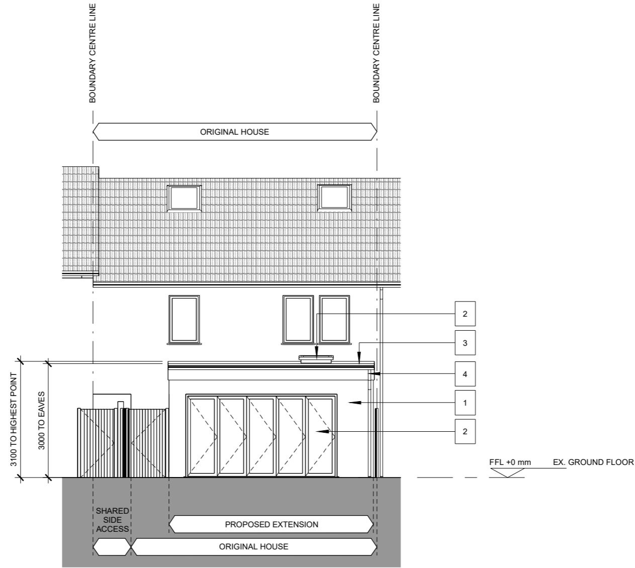
1 23095 - PROPOSED SOUTH ELEVATION 1 : 100
