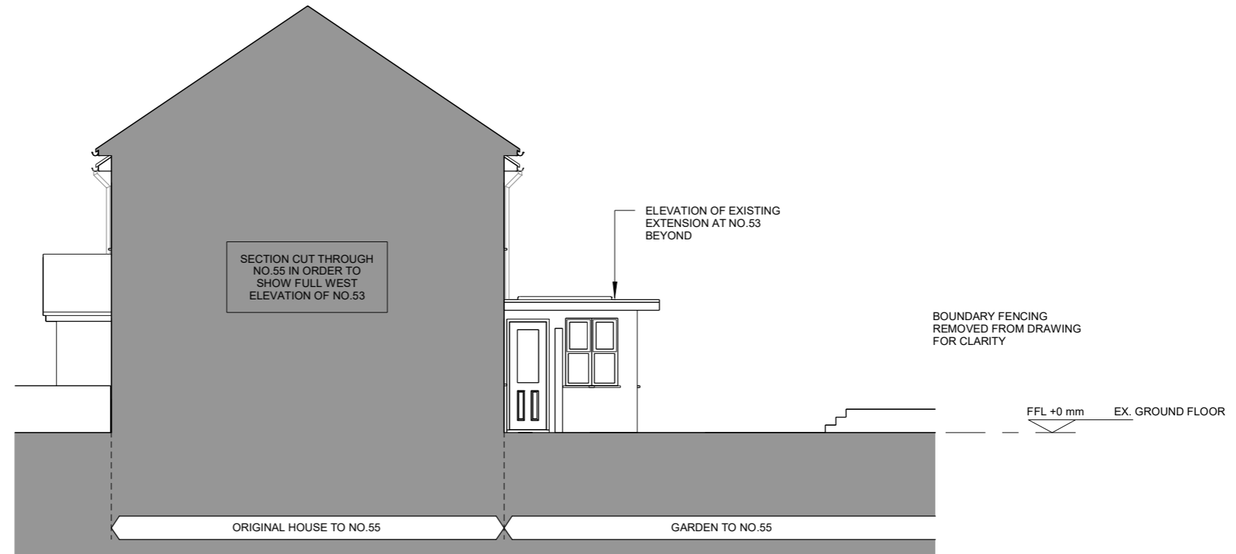
1 23095 - EXISTING WEST ELEVATION 1 : 100
