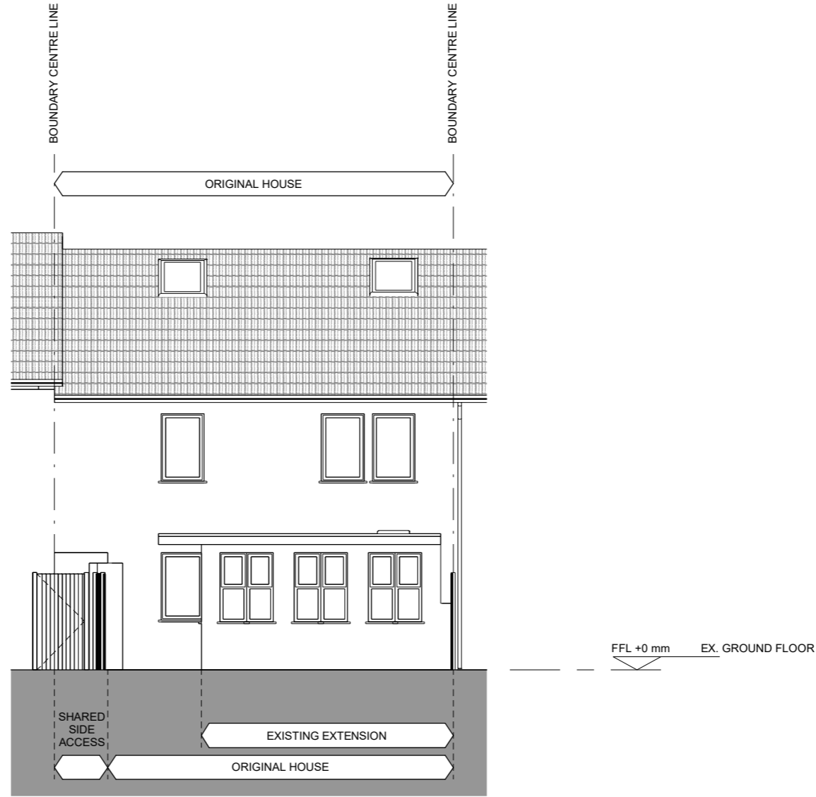
1 23095 - EXISTING SOUTH ELEVATION 1 : 100
