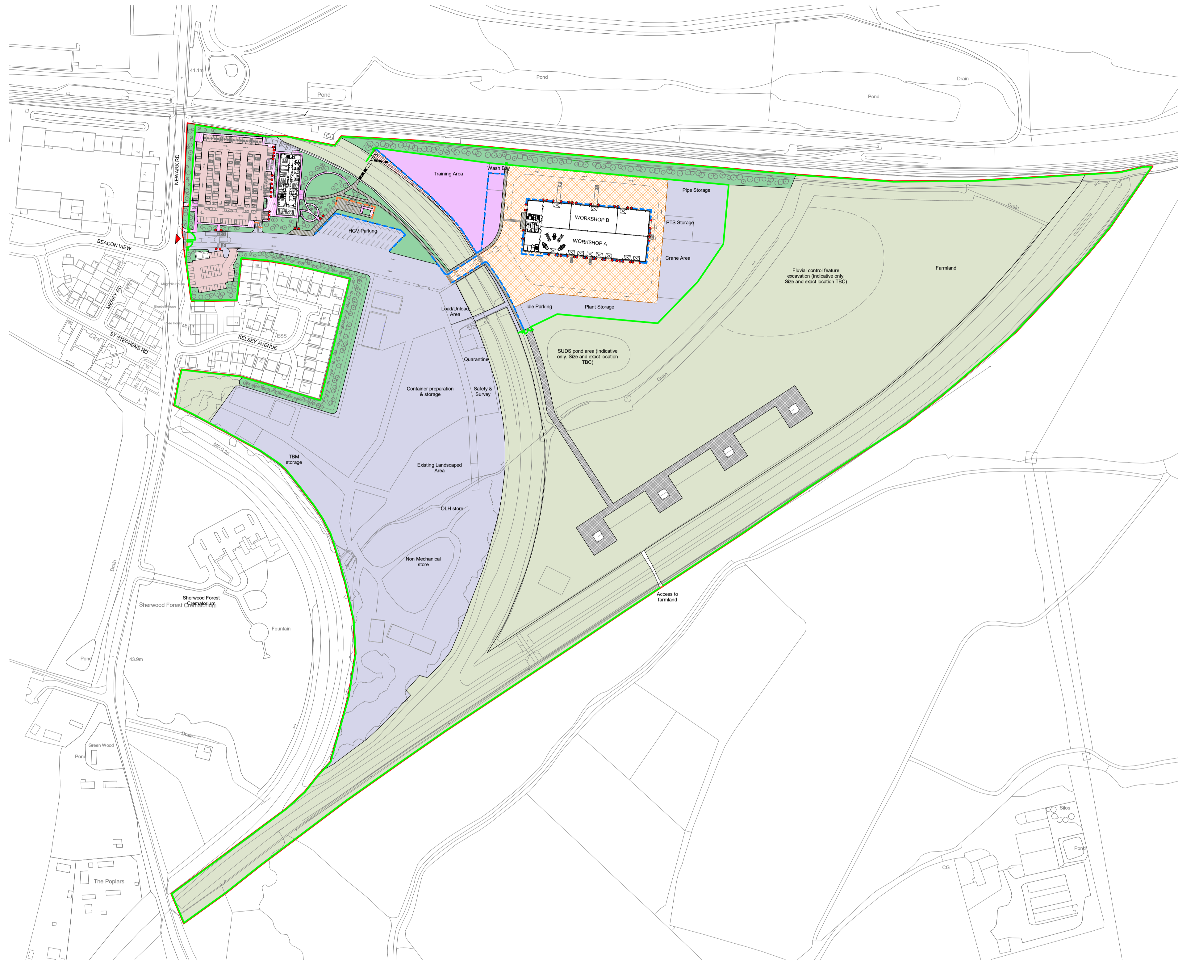
1 Site Plan - External Finishes Plan 1 : 2000
