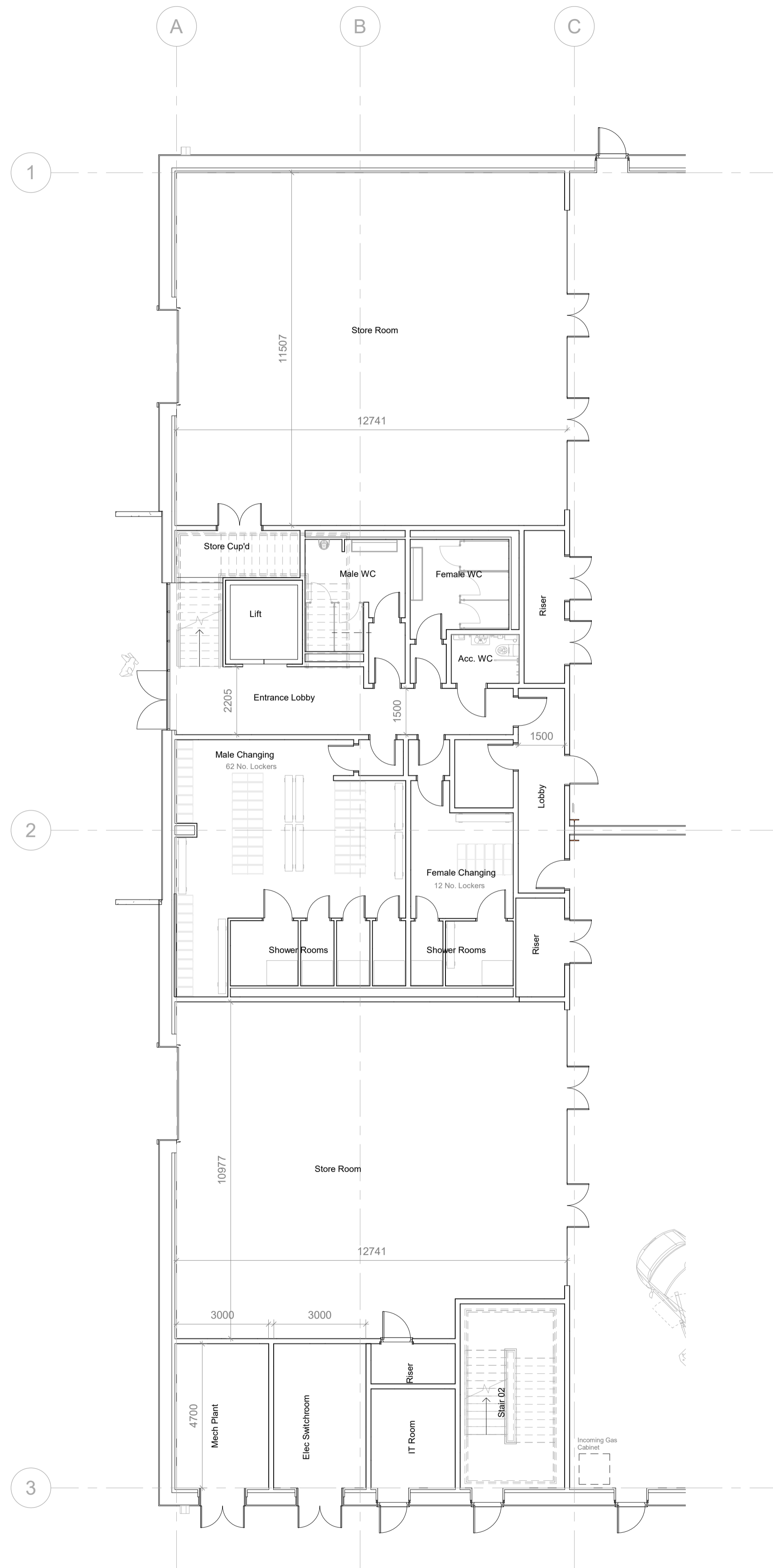
1 Ground Floor 100 1 : 100
