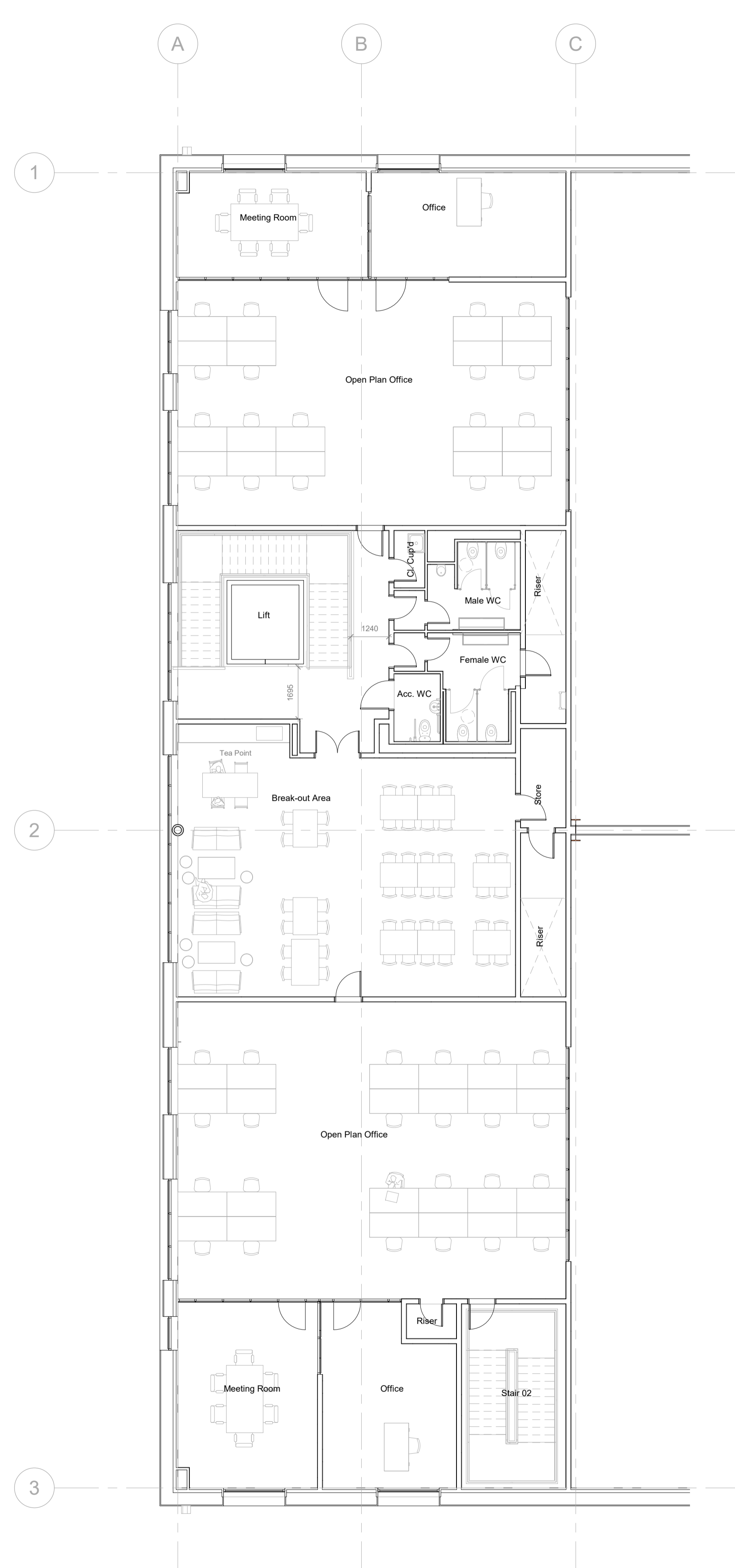
2 First Floor 100 1 : 100
