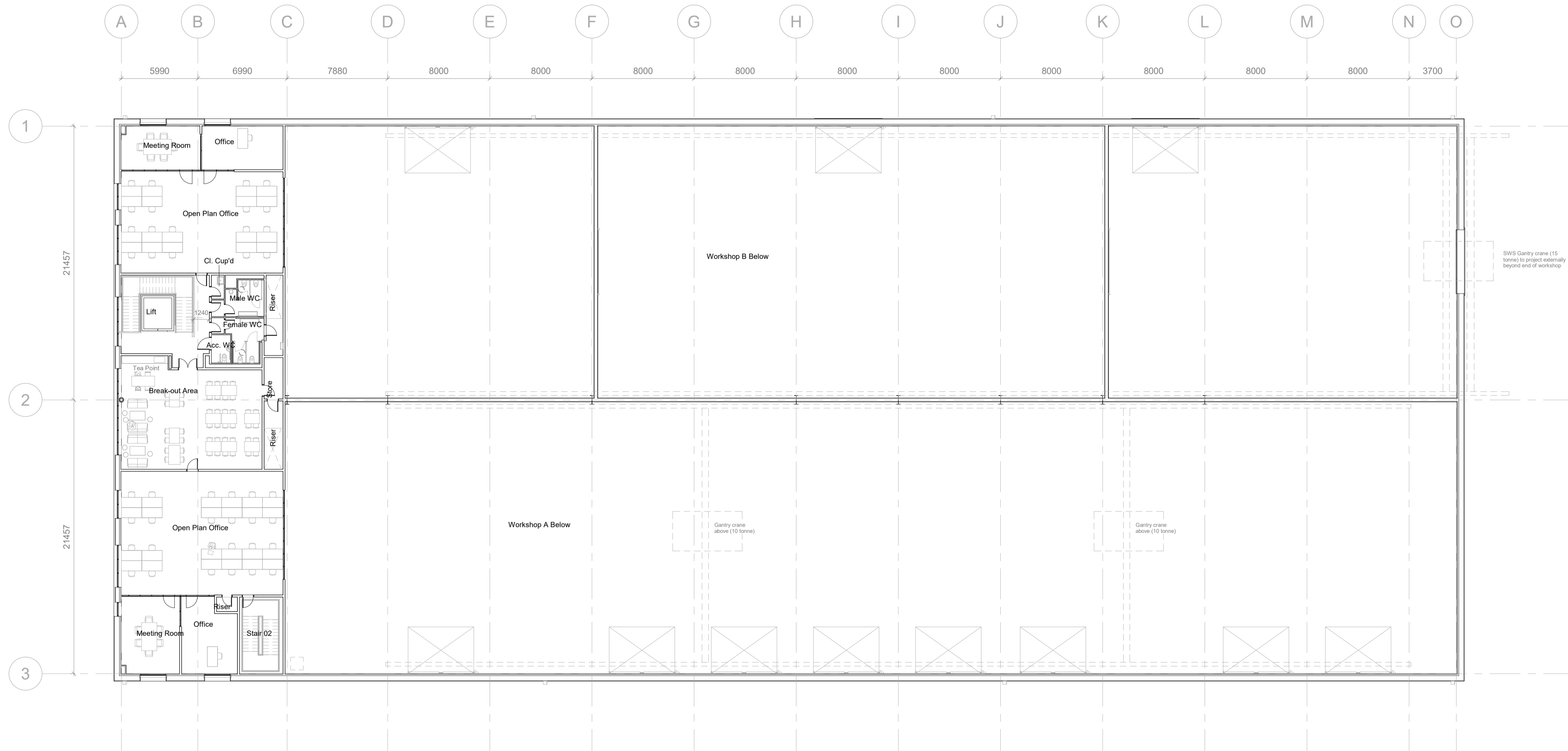
1 First Floor 1:200
