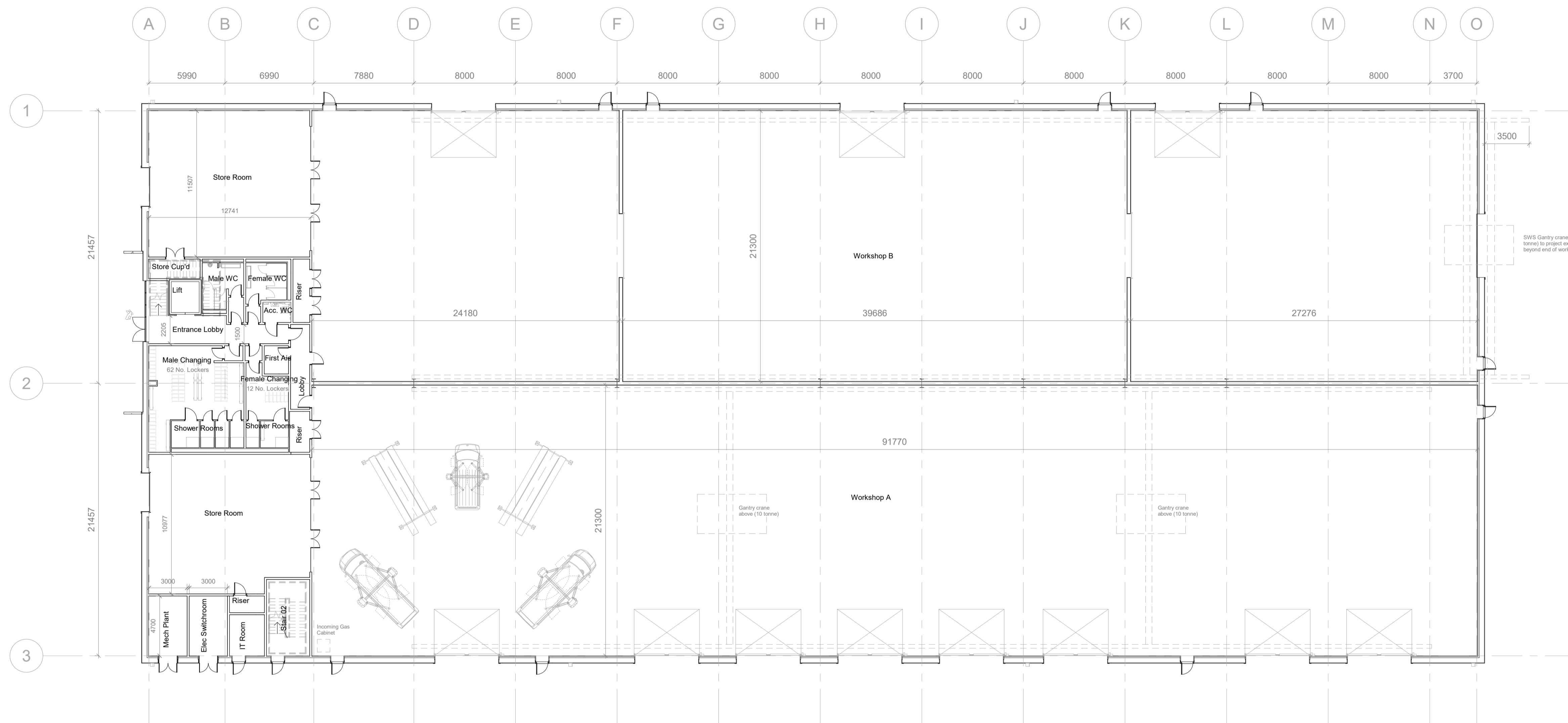
1 Ground Floor 1 : 200
