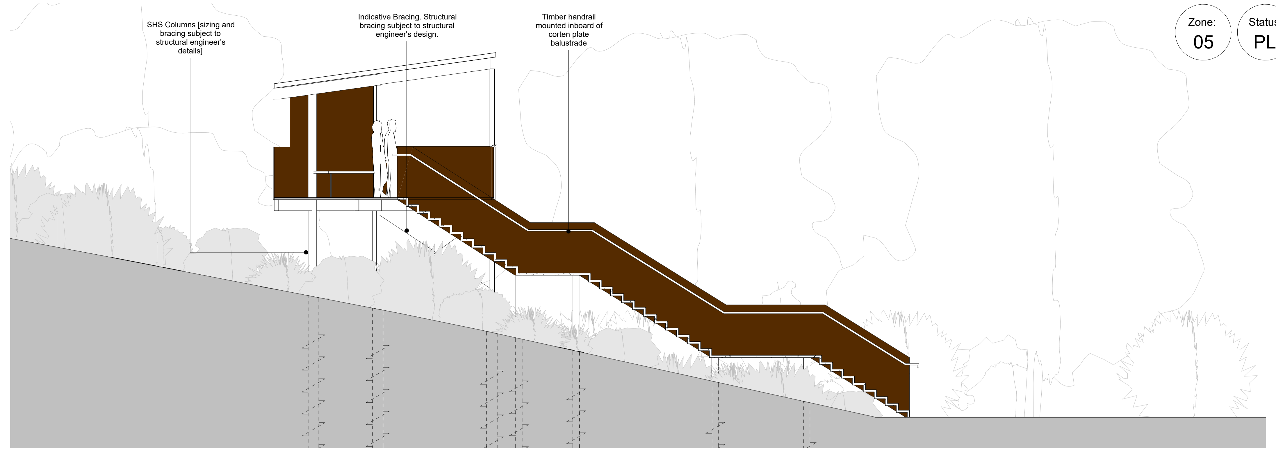
A Section A 1:50
