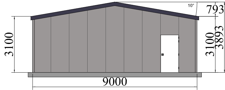
FRONT ELEVATION (EXTERNAL)
