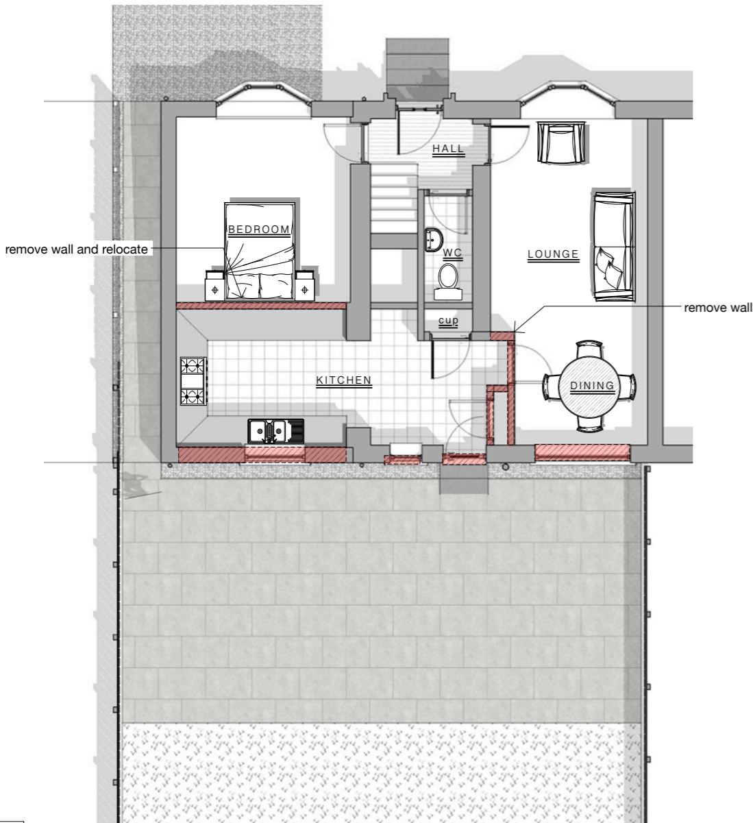
E :: EXISTING GROUND FLOOR PLAN 1 scale: 1:100
