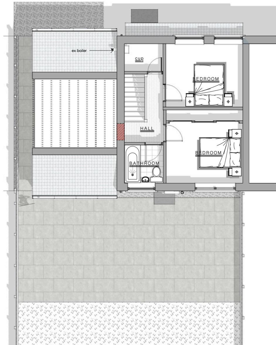
E :: EXISTING FIRST FLOOR PLAN 1 scale: 1:100
