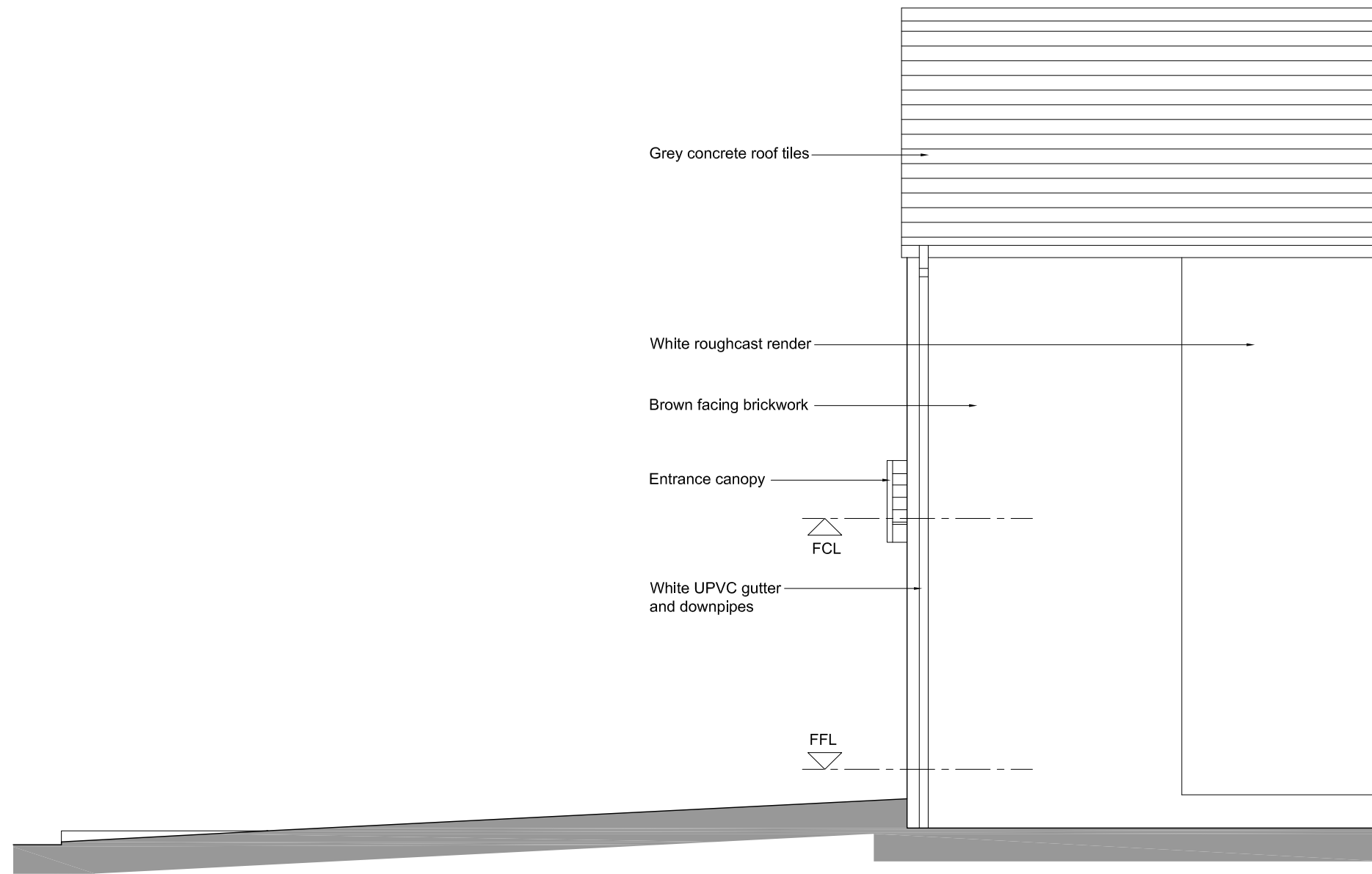
Side Elevation (East) as Existing
