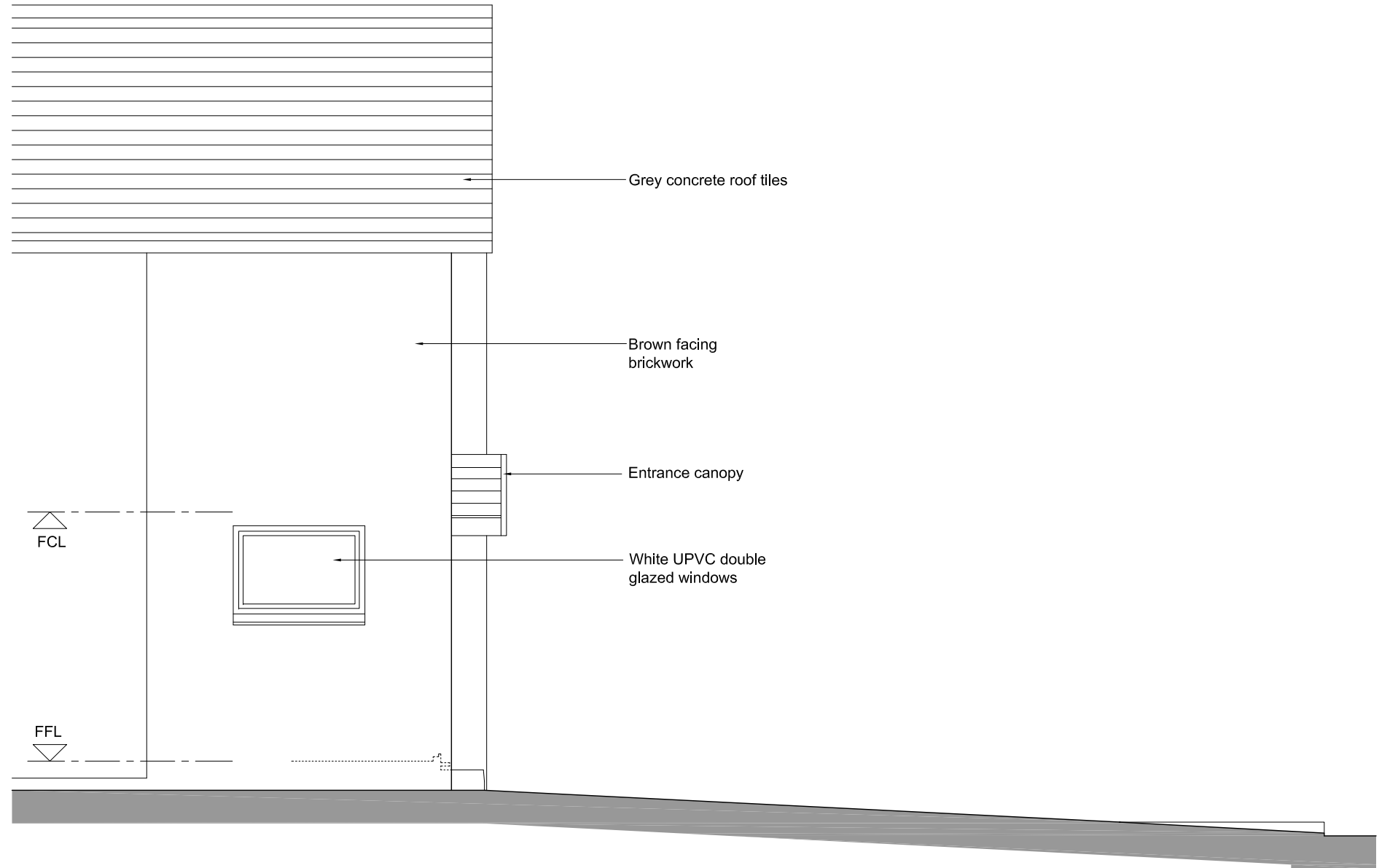
Side Elevation (West) as Existing
