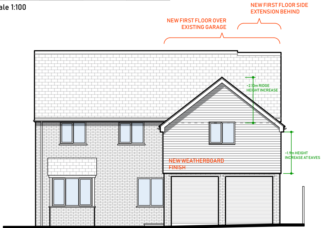
FRONT (EAST) ELEVATION
