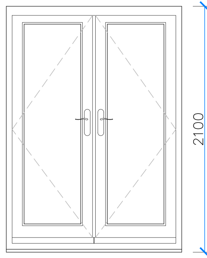
Proposed Door Elevation Scale 1:20
