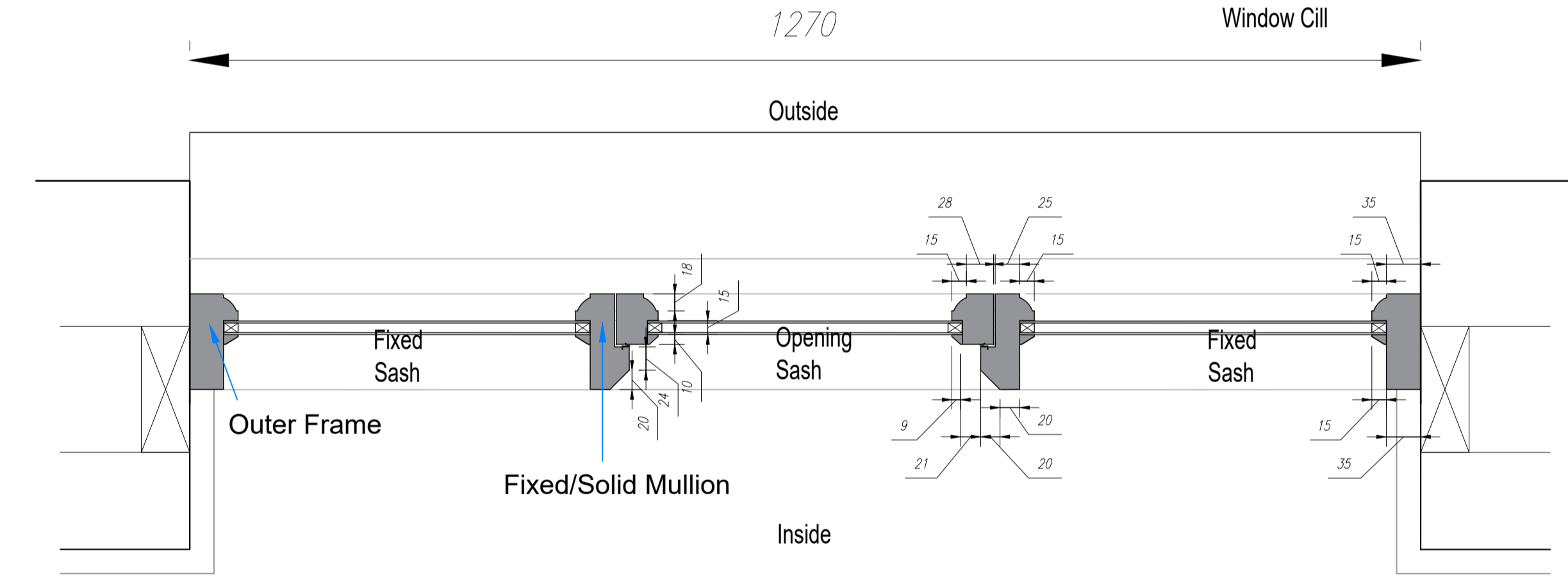
Proposed Window Detail Scale 1:5
