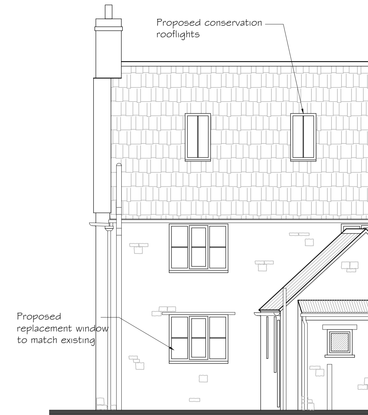
Details of the new window W-01 (not to scale)
