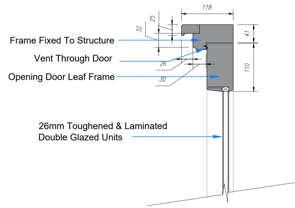
Proposed Door Section (Top) Scale 1:5
