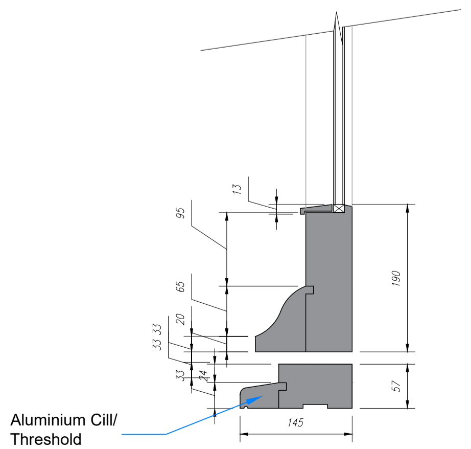
Proposed Door Section (Bottom) Scale 1:5
