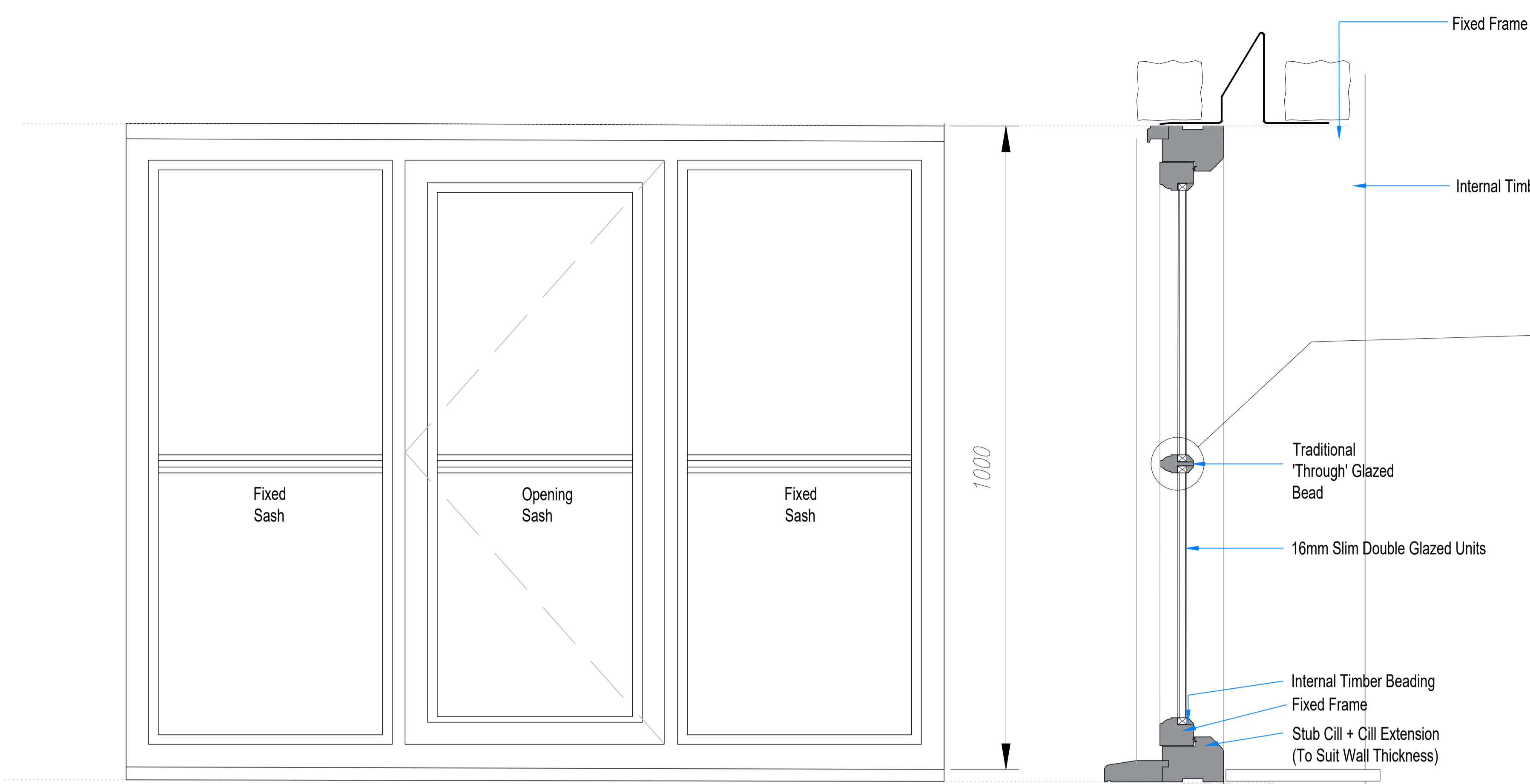
Proposed Glazing Bar Detail Scale 1:5
