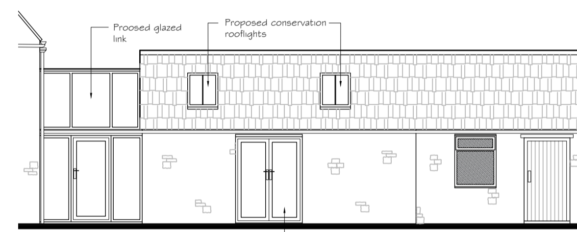
Details of the new doors D-01 (not to scale)
