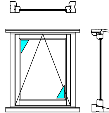
REAR ELEVATION UTILITY ROOM WINDOW
