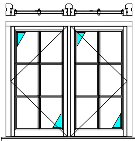
FRONT ELEVATION ATTIC LEFT & RIGHT DORMER WINDOWS
