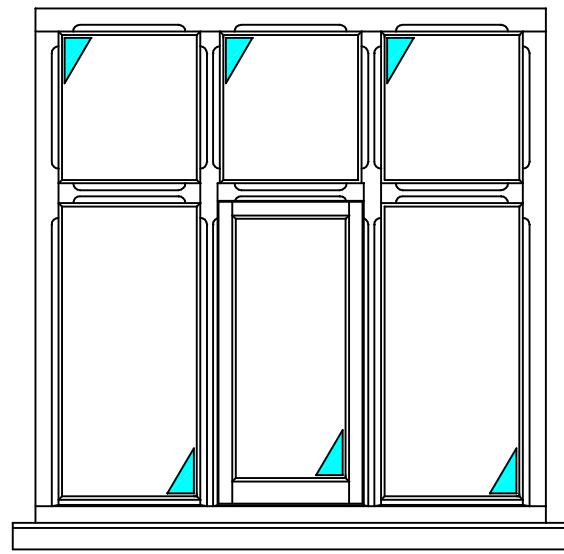
FRONT ELEVATION GROUND FLOOR WINDOW
