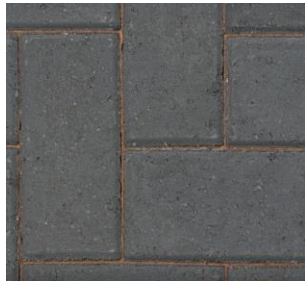
By: Marshalls Product: Key Block Paving Colour: Charcoal
