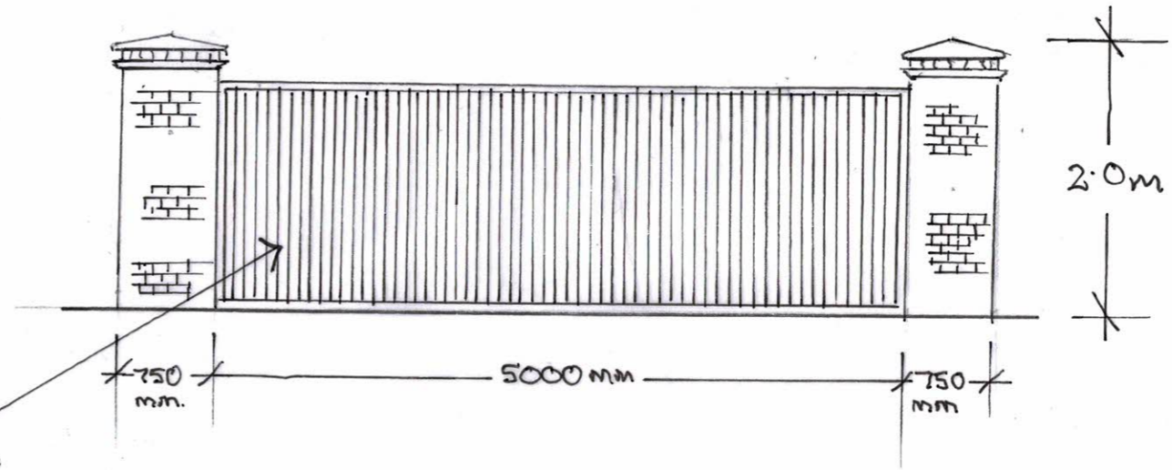
BRICK PILLARS & TIMBER GATE
