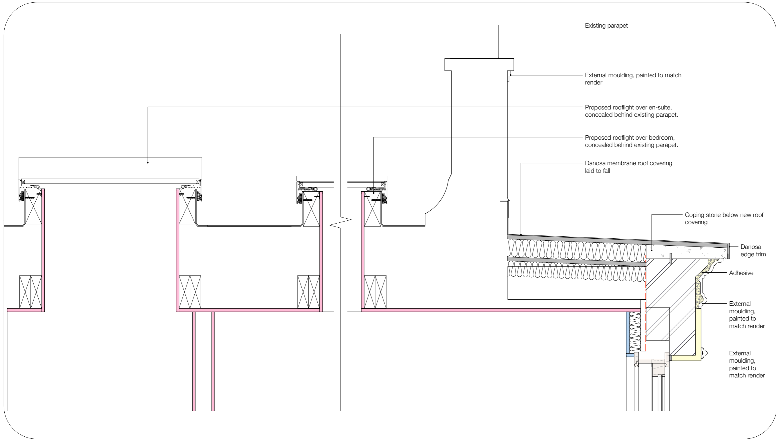
SECTION THROUGH FLAT SKYLIGHTS, EXISTING PARAPET TO FRONT OF EXISTING HOUSE, AND SECTION THROUGH DECORATIVE DETAILS OF BAY WINDOW
