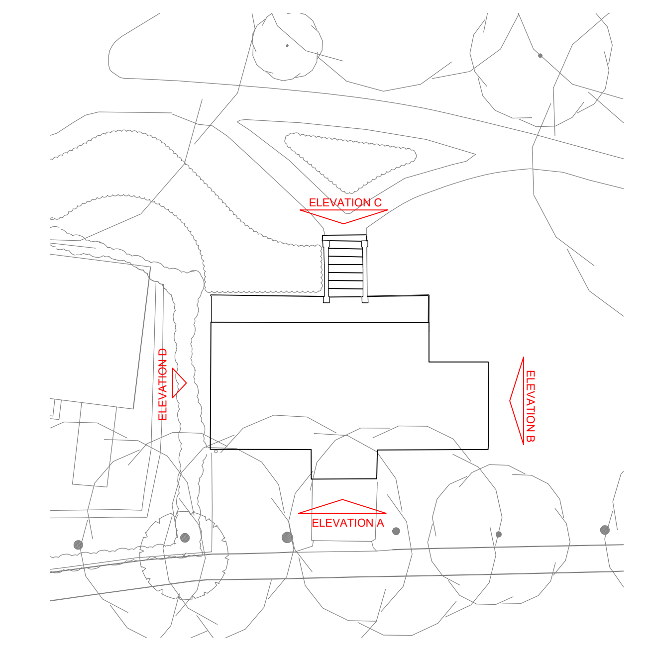
Keyplan NTS
