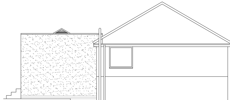
EAST ELEVATION
