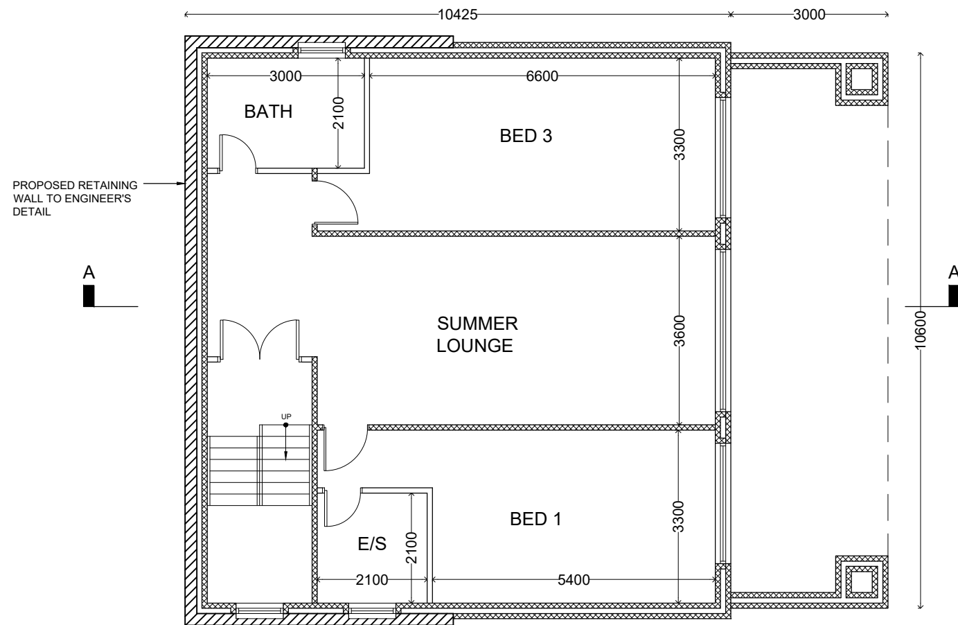
LOWER GROUND FLOOR PLAN
