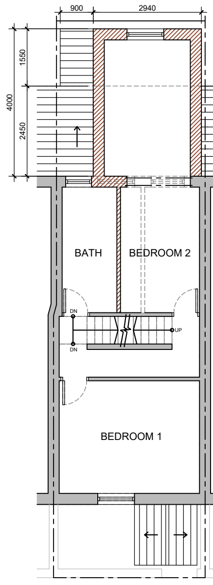
FIRST FLOOR PLAN 1:100 Scale 1:100
