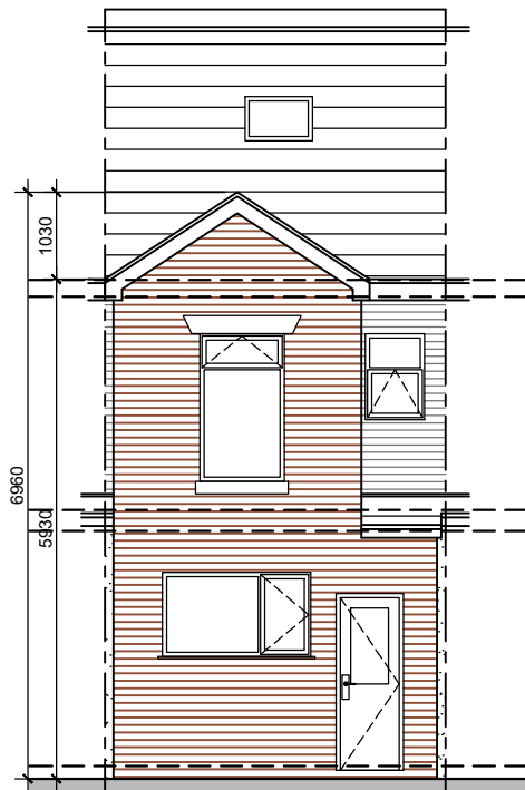
REAR ELEVATION 1:100
