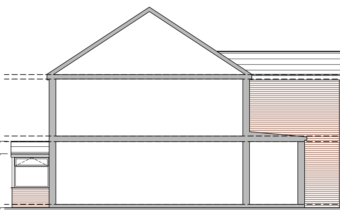
RIGHT ELEVATION 1:100
