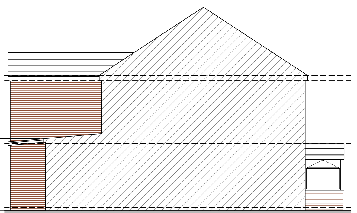
LEFT ELEVATION 1:100
