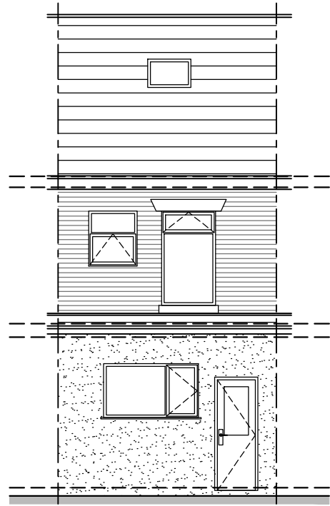
REAR ELEVATION
