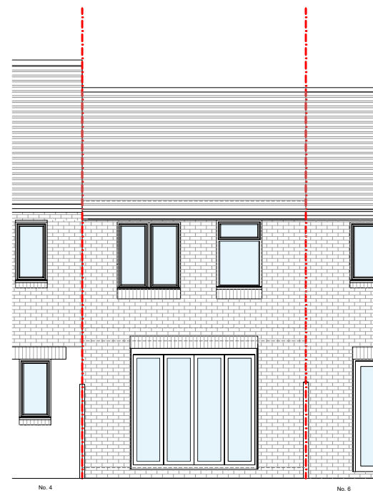
A EXISTING ELEVATION A
