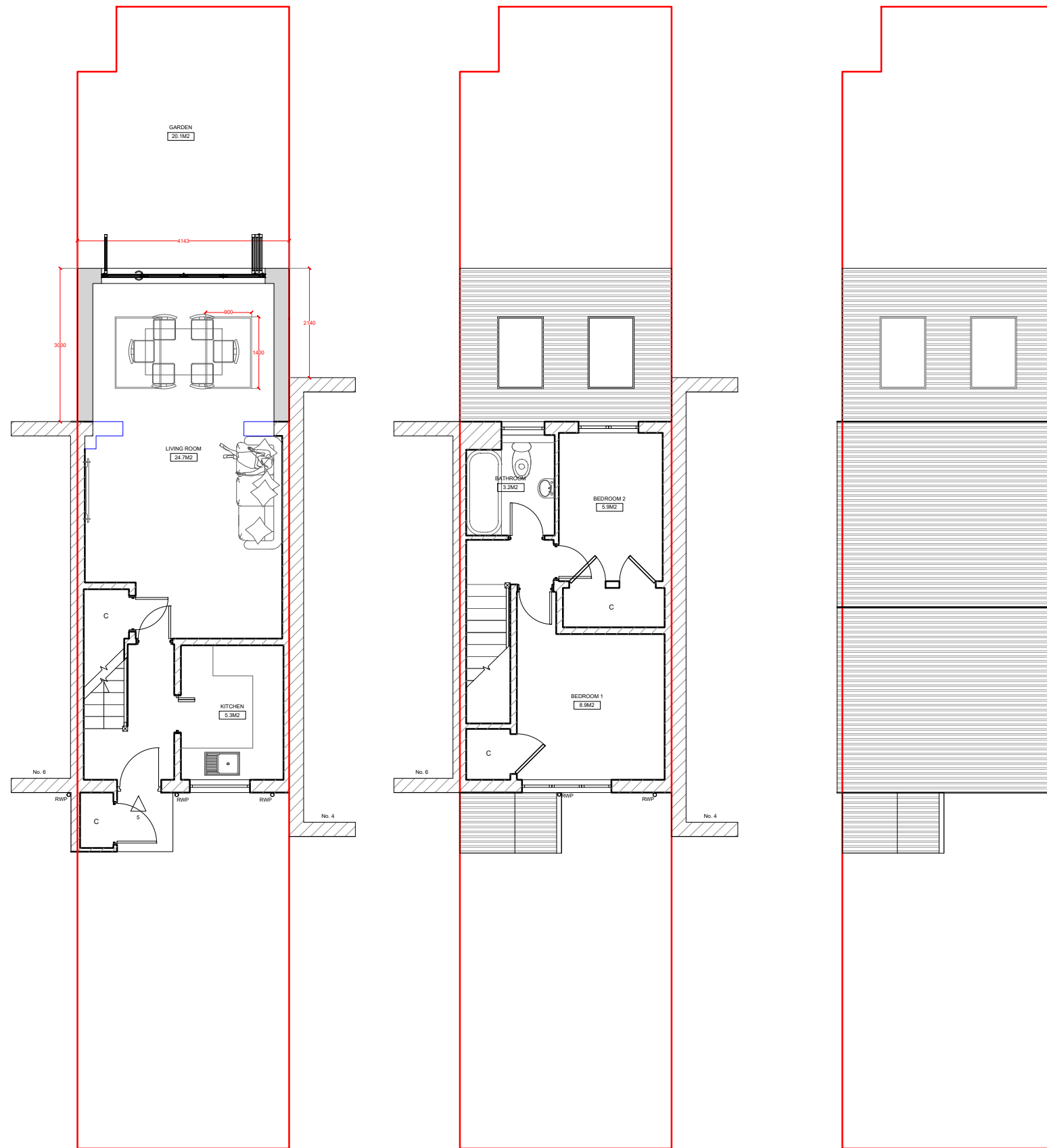
Ⓒ PROPOSED GF PLAN
