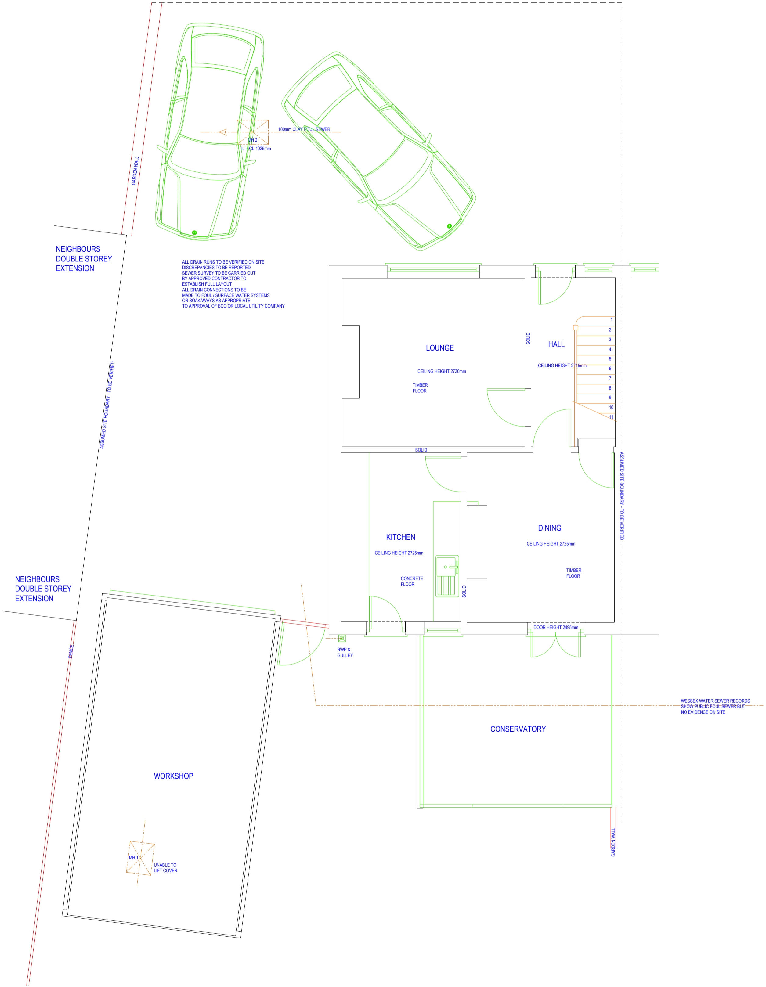
EXISTING GROUND FLOOR PLAN 1:50 @ A2
