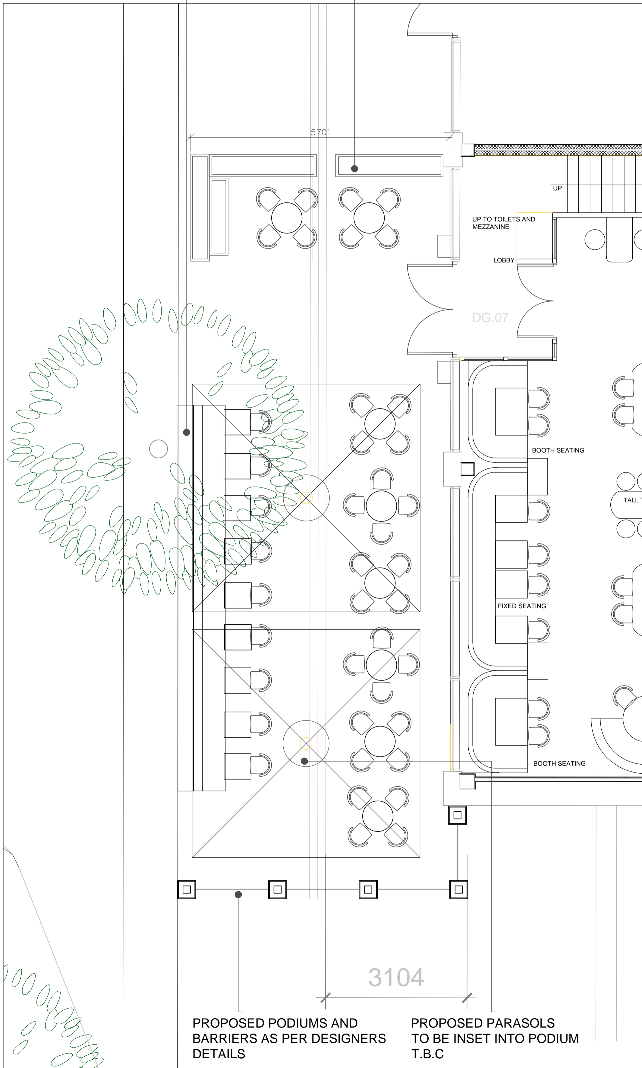
PROPOSED WINTER LAYOUT SCALE 1:50 50 COVERS
