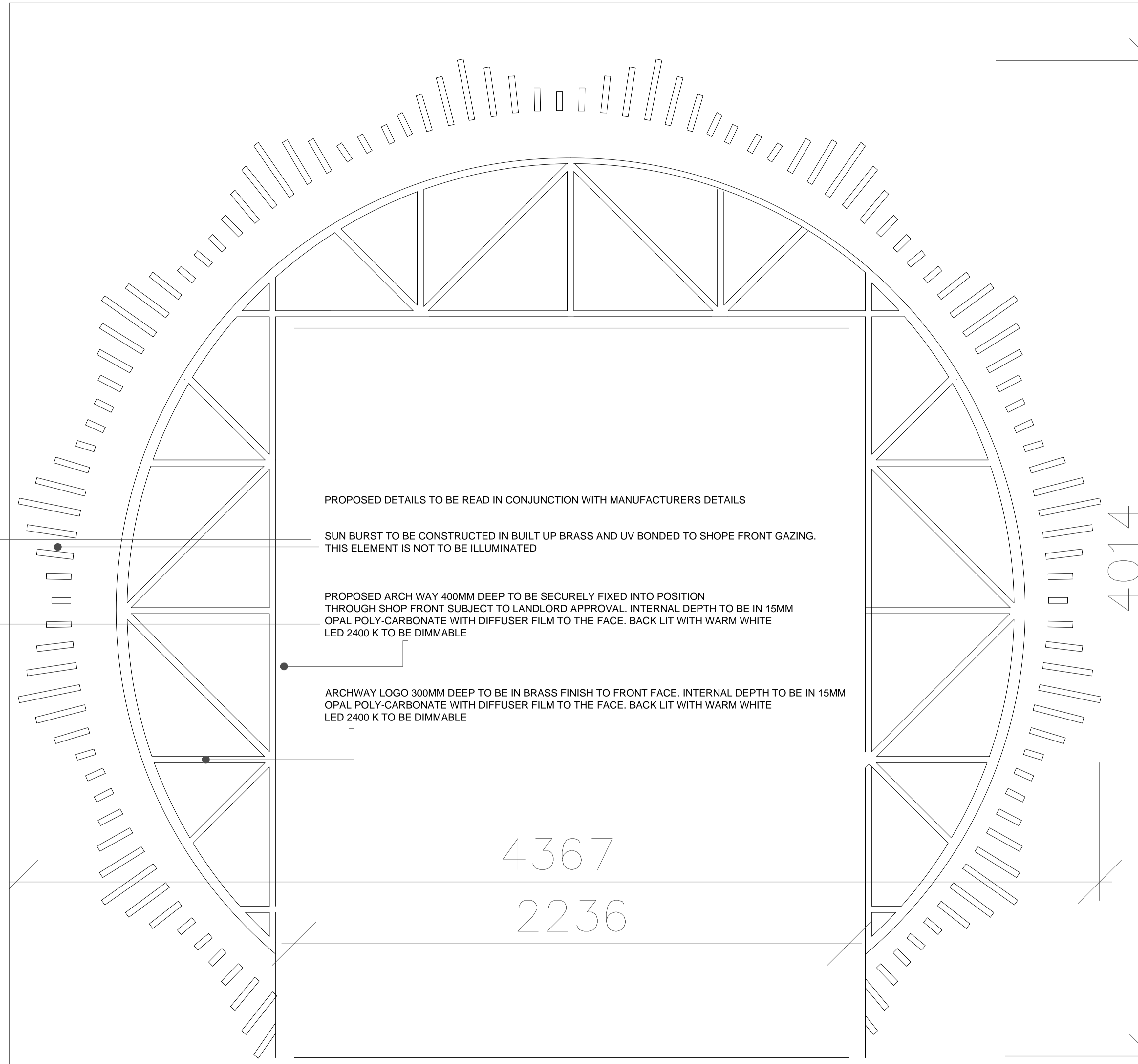
PROPOSED FEATURE LIT ARCH ELEVATION SCALE 1:5
