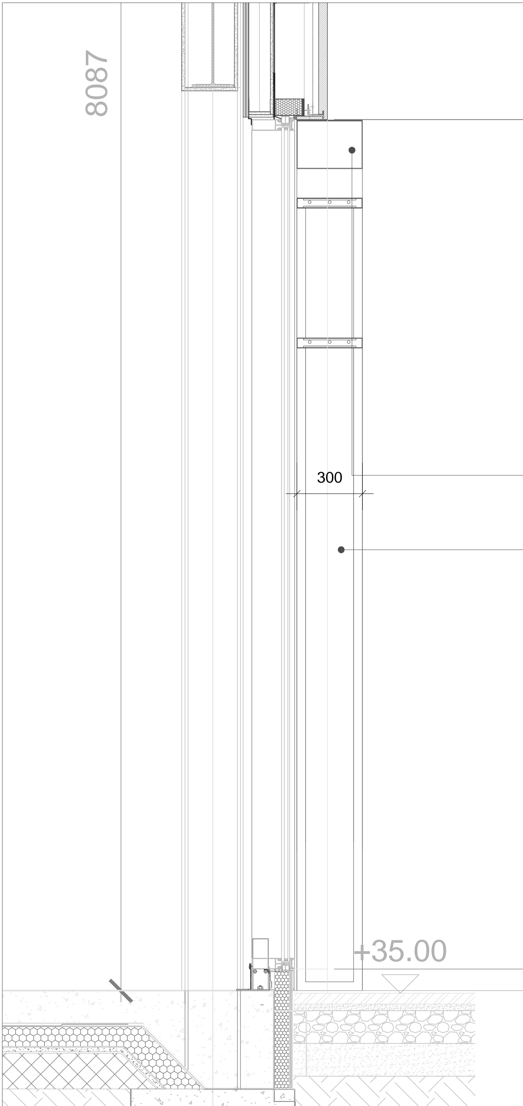
PROPOSED FEATURE LIT ARCH SECTION SCALE 1:5
