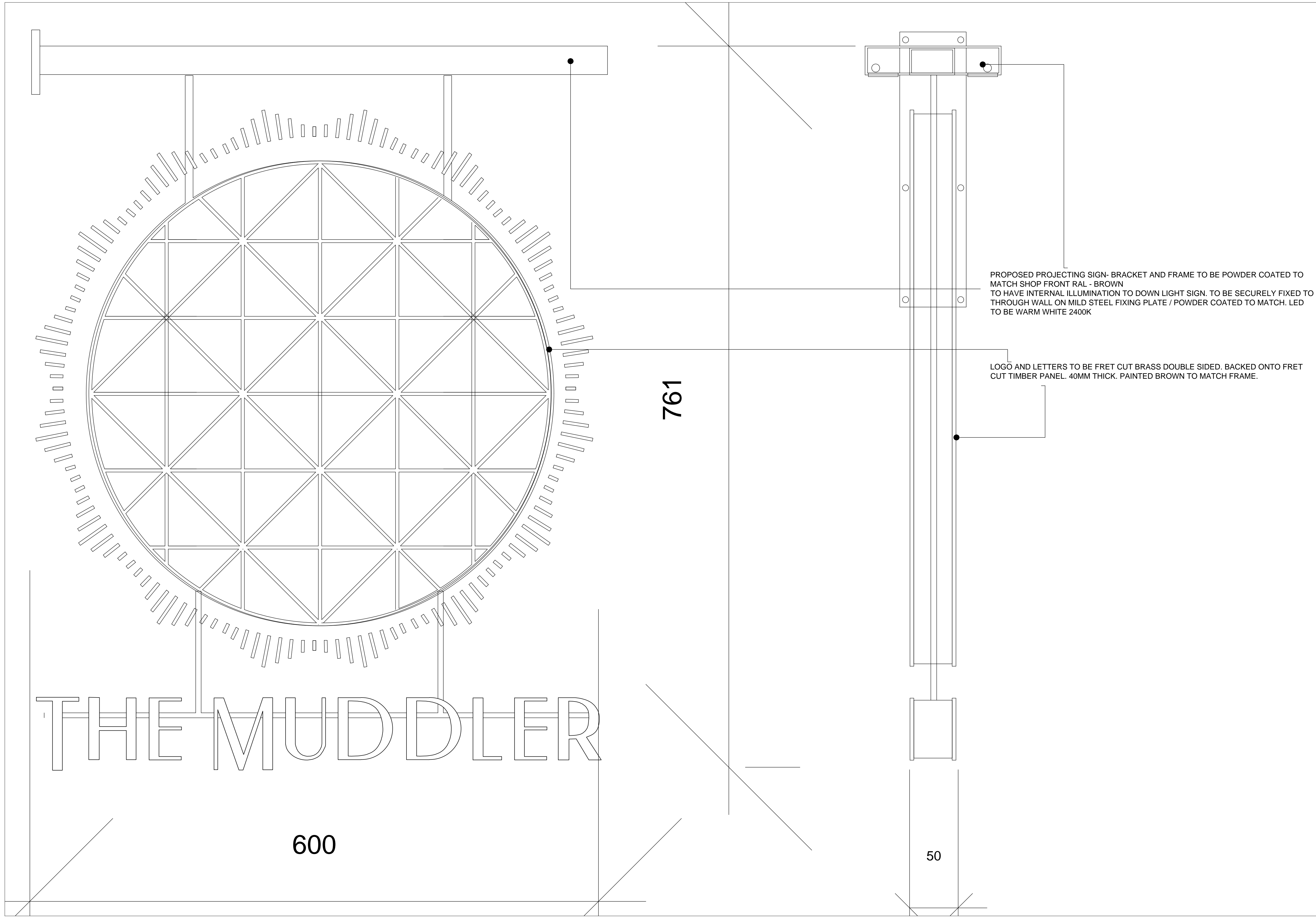
PROPOSED ELEVATION SCALE 1:2
