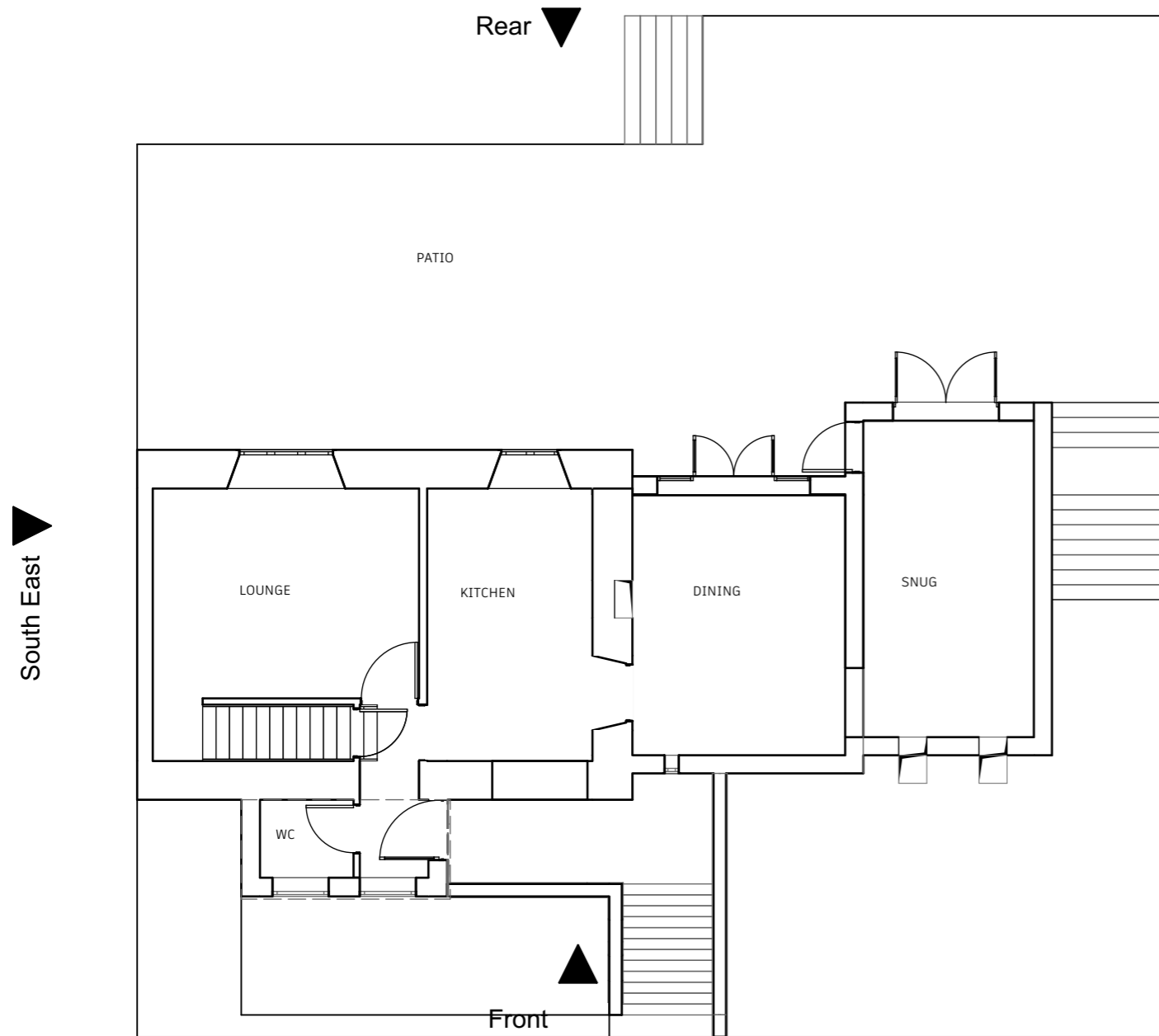
1:100 EXISTING GROUND FLOOR GENERAL ARRANGEMENT
