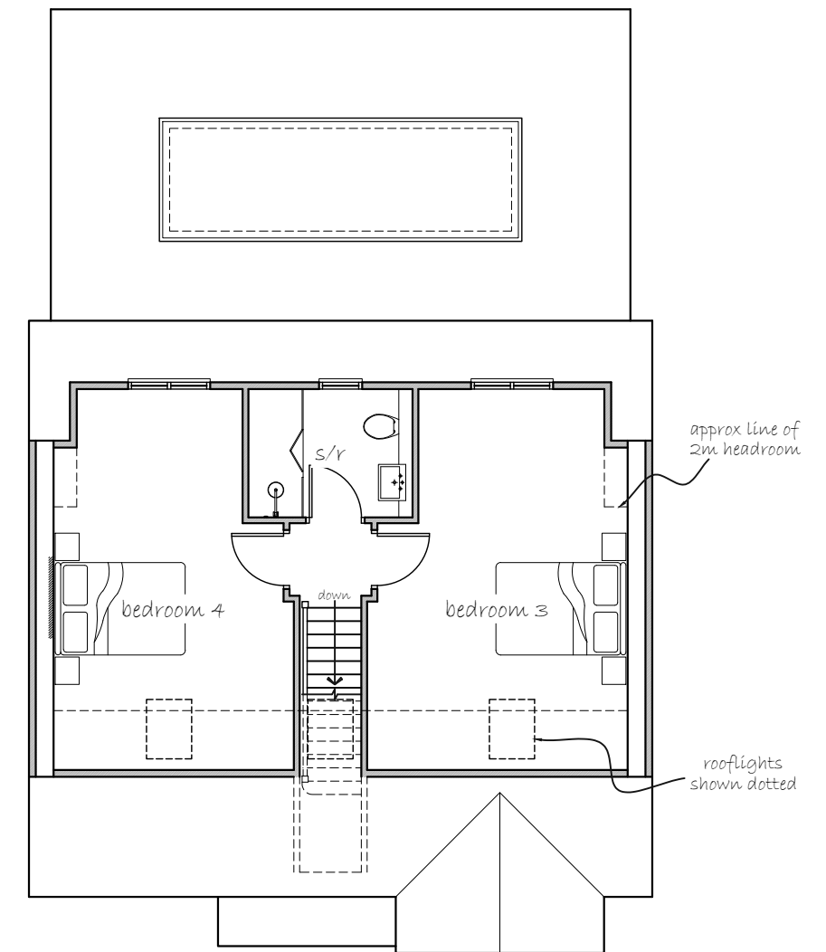
Proposed Second Floor Plan - 1:100
