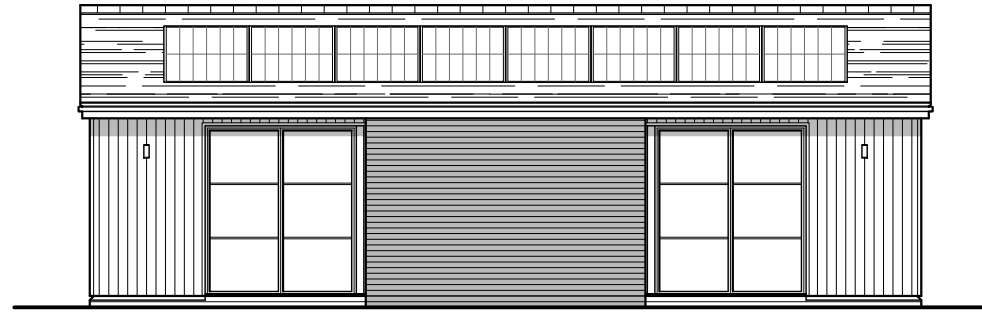
Proposed South-East Elevation - 1:100
