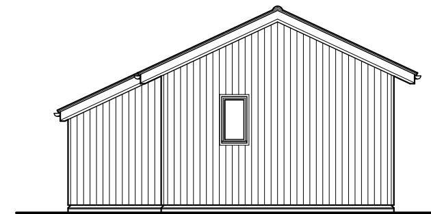
Proposed South-West Elevation - 1:100
