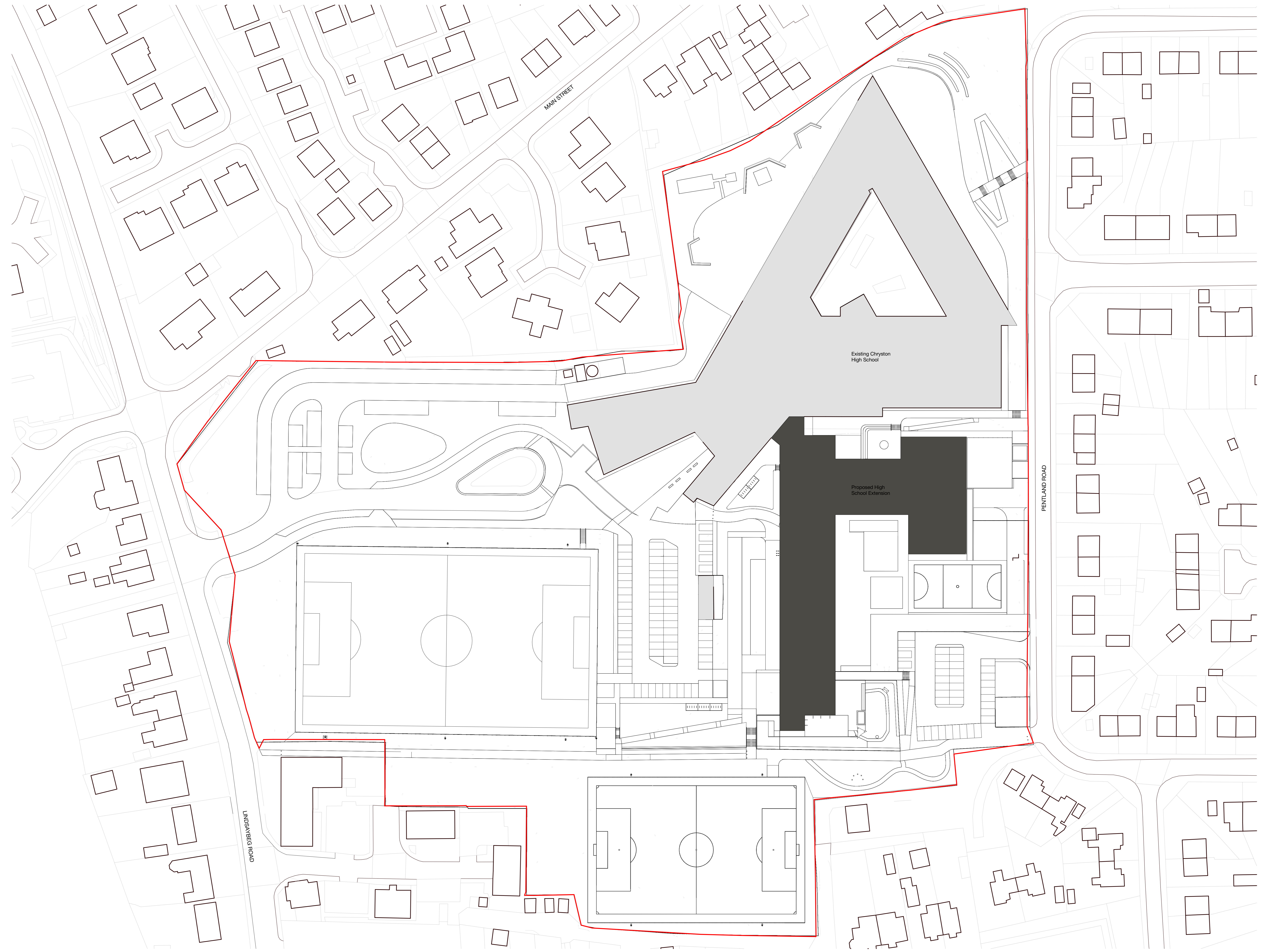
1 Block Plan 1_500 1:500
