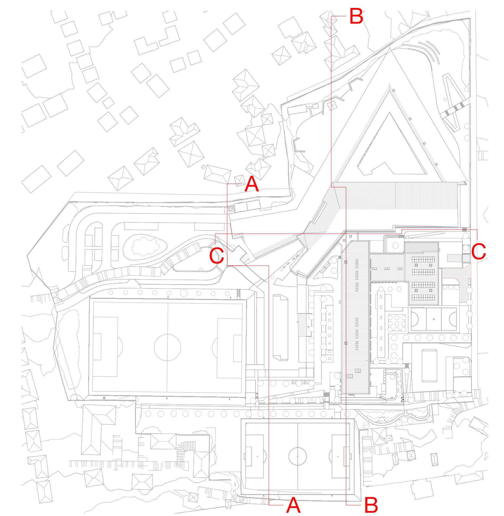
4 Key Plan 1:1500
