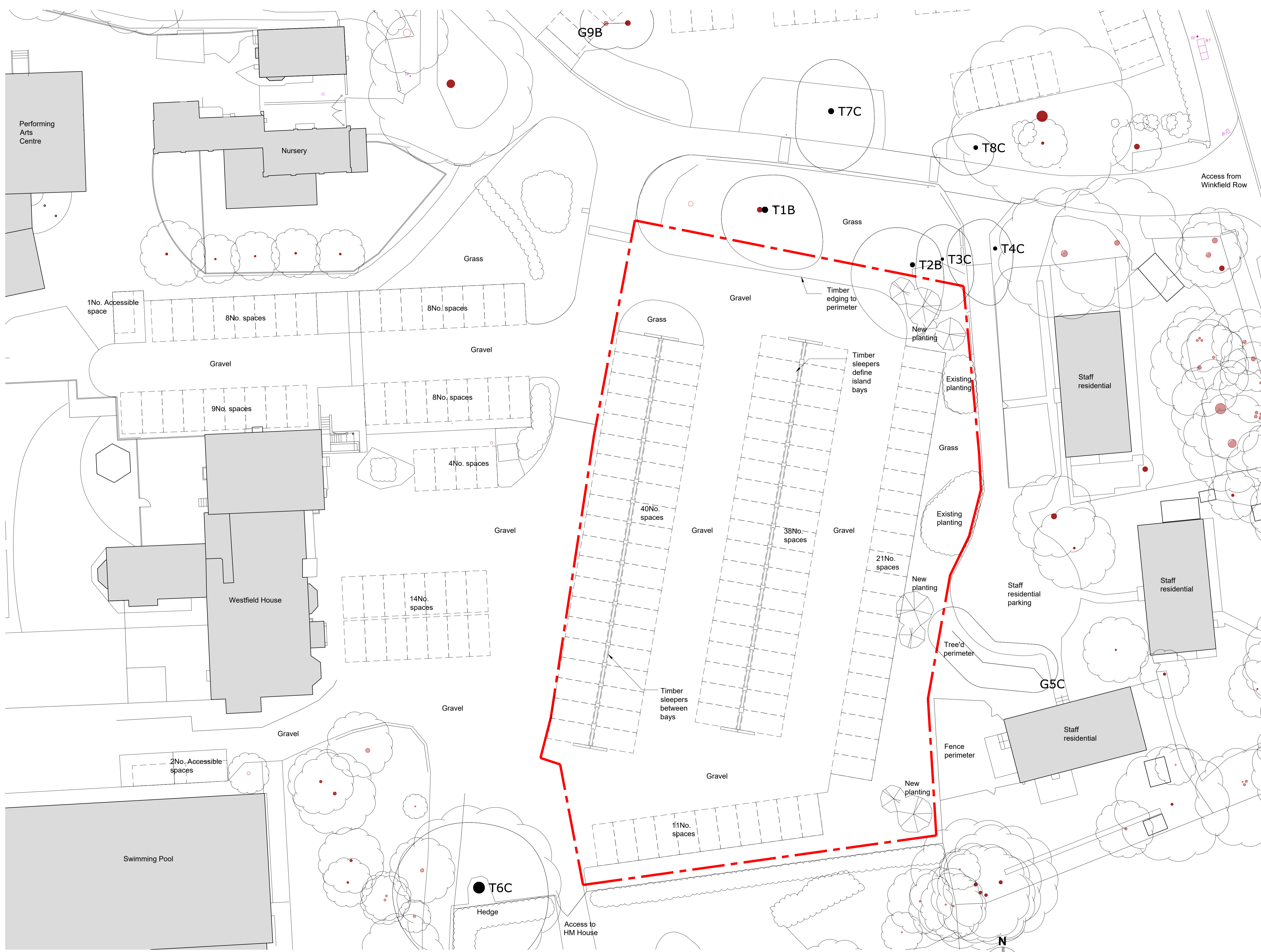
01 Proposed Layout Plan 1:200
