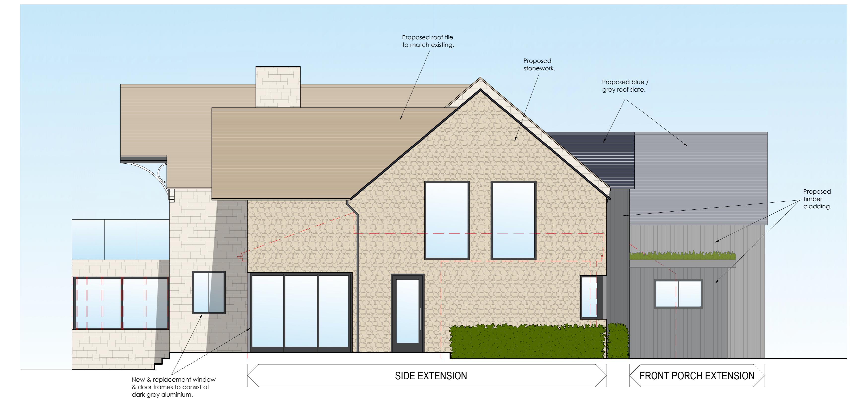
Proposed Southwest (Side) Elevation Scale 1:50
