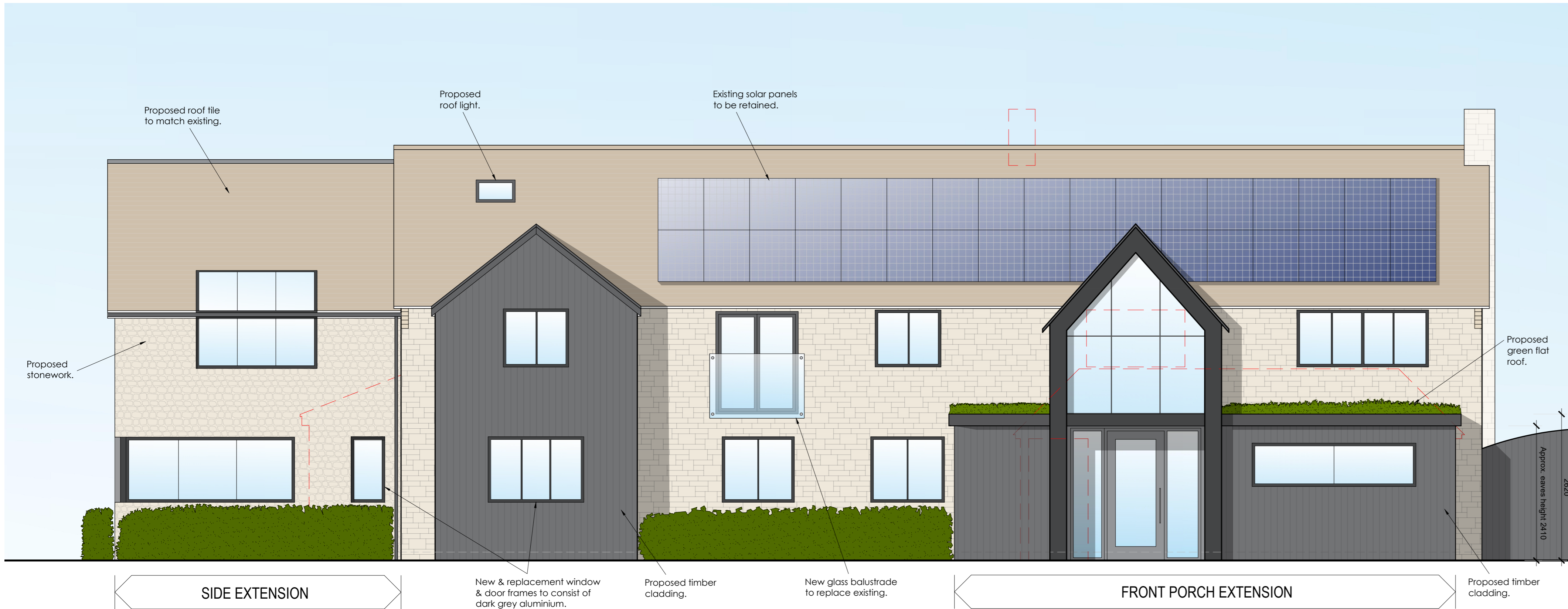
Proposed Southwest (Front) Elevation Scale 1:50
