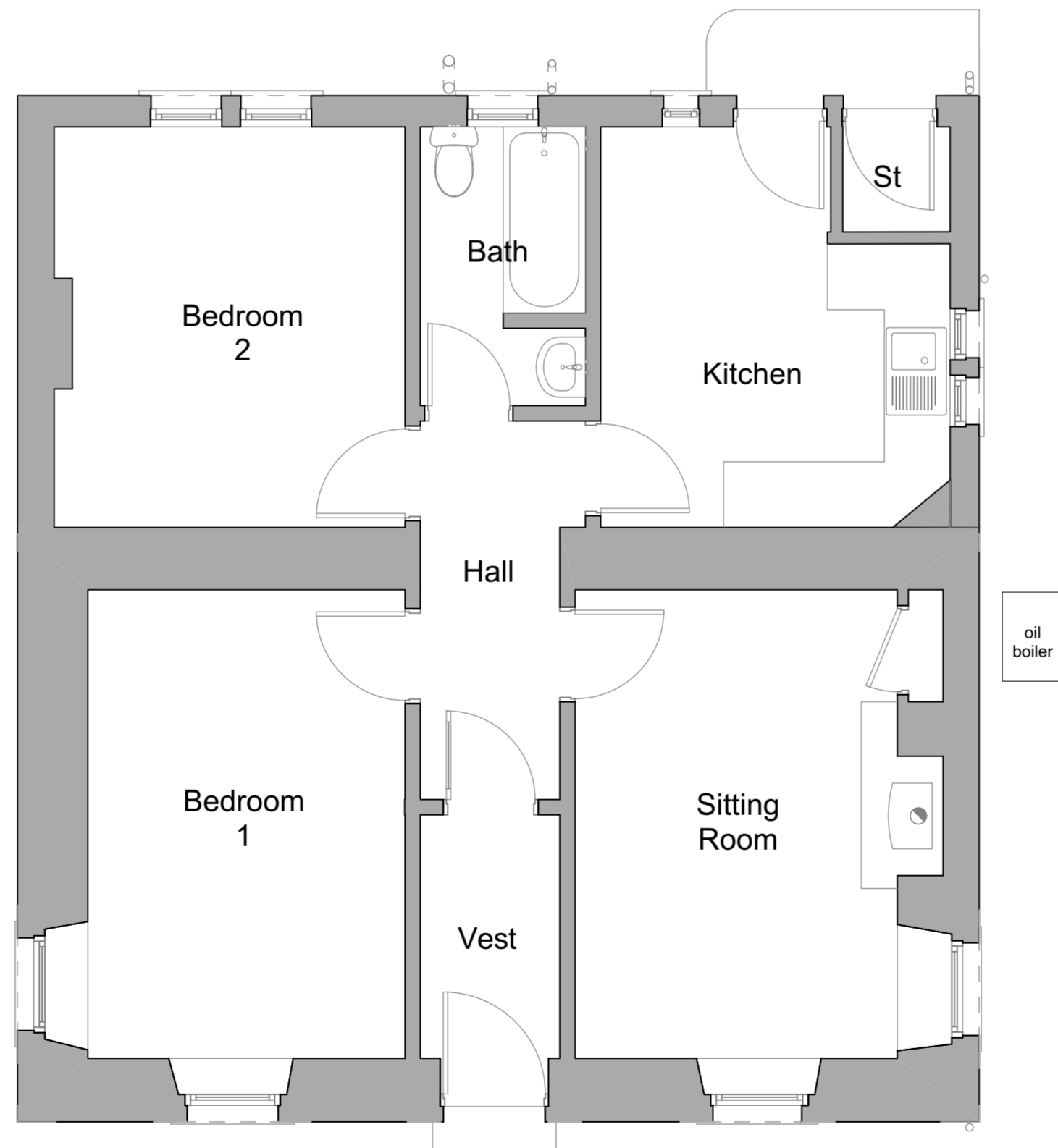
Floor Plan 1:50
