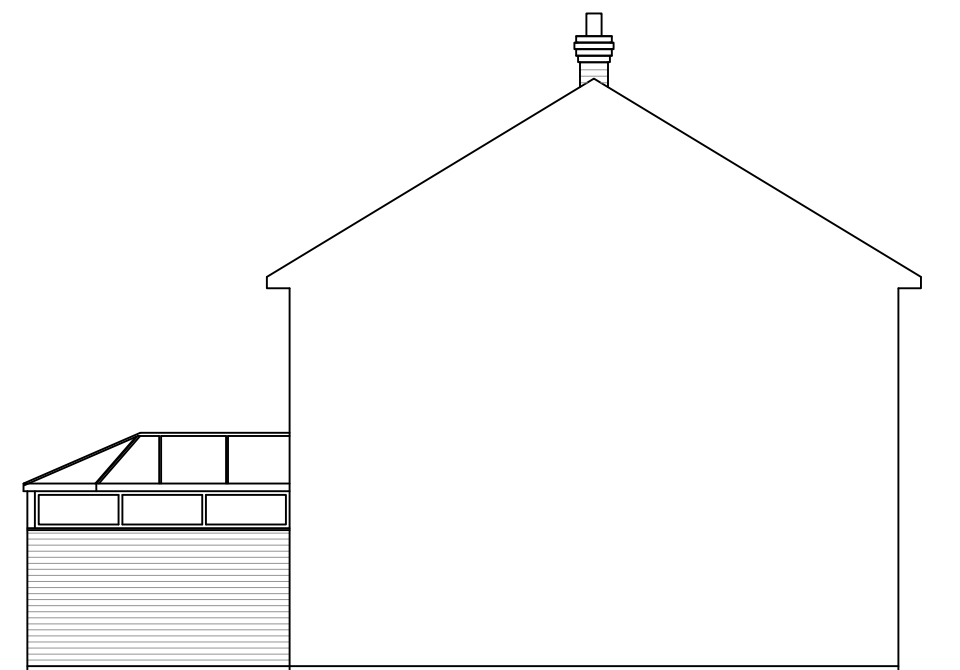
SIDE ELEVATION
