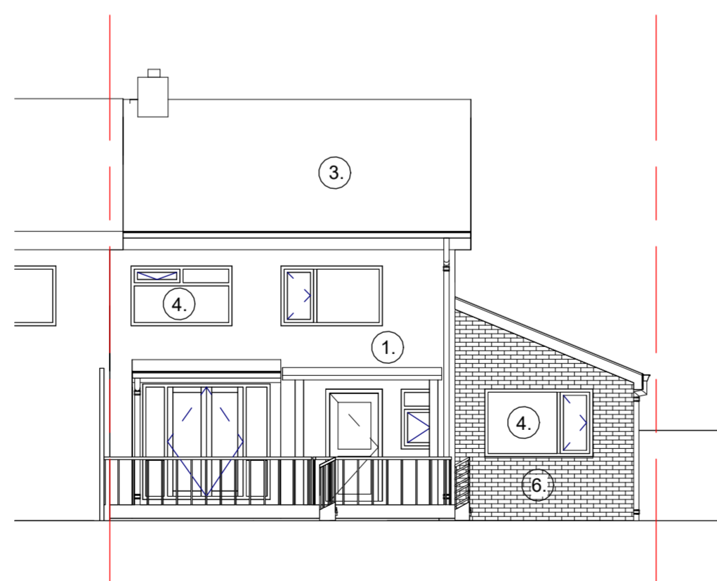
South Elevation (Back)
