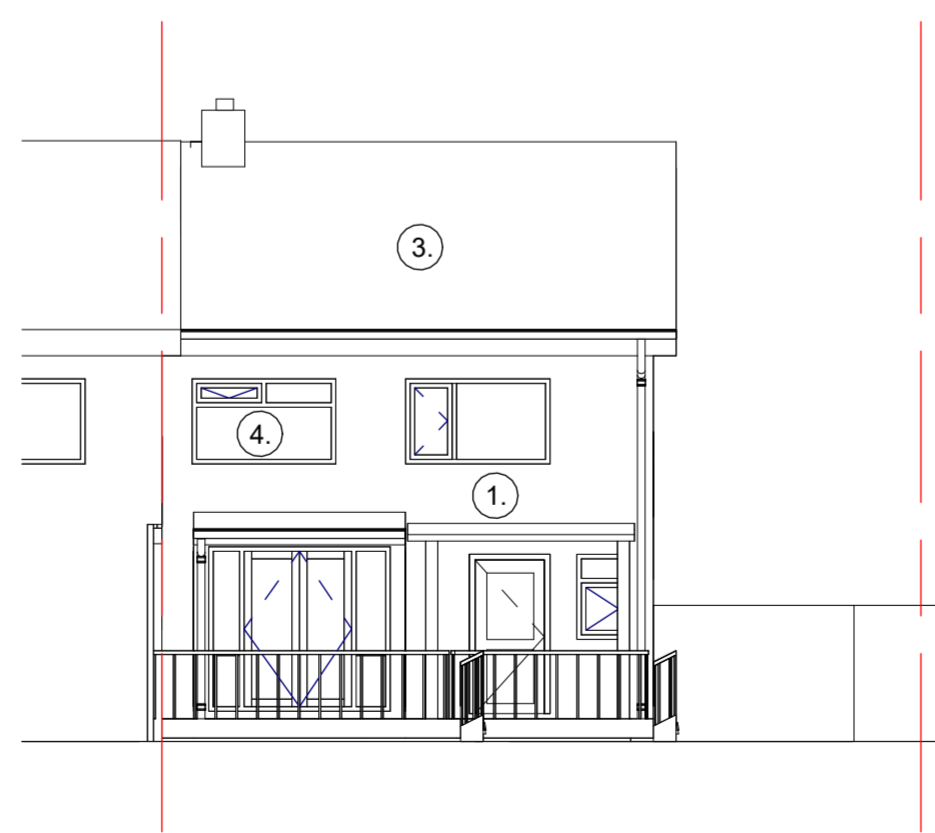
South Elevation (Back)
