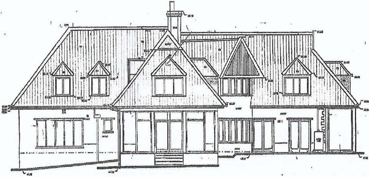
WEST ELEVATION
